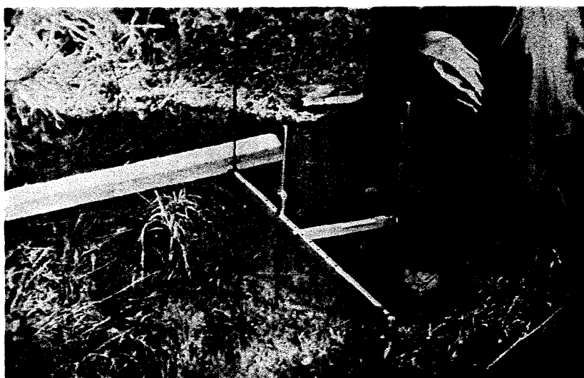
Figure 1. --Measuring the distance from the metal crossbar to mineral soil at one of the '74 erosion stations.
