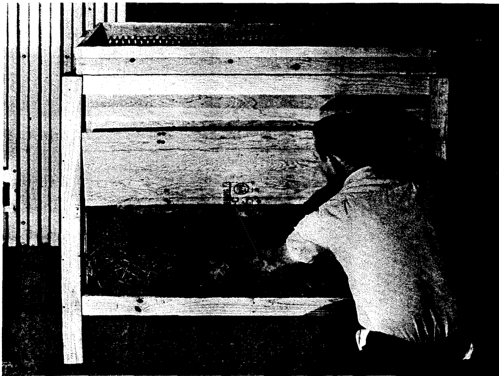
Figure 1.--Technician removes a completed fuel bed from the bottom of the fuel bed fabricator. Note the arrangement of the rods which make up the grate.
