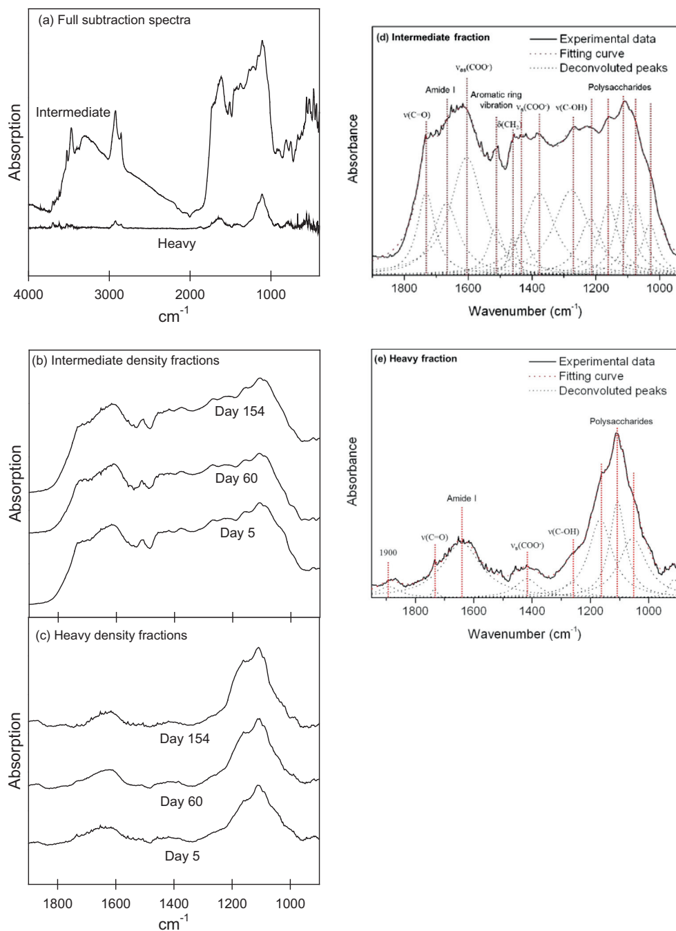
Fig. 3. DRIFT subtraction spectra of density fractions. The DRIFT spectrum of pure gibbsite was subtracted from each density fraction spectrum. (a) Full spectra from 400–4000 \text{cm}^{-1} of a representative intermediate and heavy fraction. (b) Intermediate density fractions from 900–1900 \text{cm}^{-1} . (c) Heavy density fractions from 900–1900 \text{cm}^{-1} . (d) and (e) illustrate the peak deconvolution and peak assignments for the intermediate and heavy fractions.
