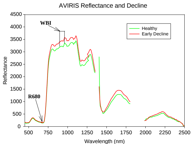
Fig. 5. AVIRIS data extends from 450 to 2500 nm with strong atmospheric water absorption bands removed and reflectance averaged for healthy samples ( \text{Decline} < 2 ) and those experiencing the early stages of decline ( 2 < \text{Decline} < 4 ). We highlight those wavelengths found to be significant in predicting hemlock decline.
