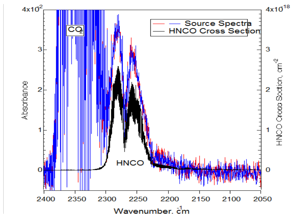
Figure 11.1 Two consecutive infrared spectra of HNCO source output (red, blue) and PNLL reference spectrum (black) as used to quantify the mixing ratio of isocyanic acid during the 2009 Fire Sciences Lab burns.
