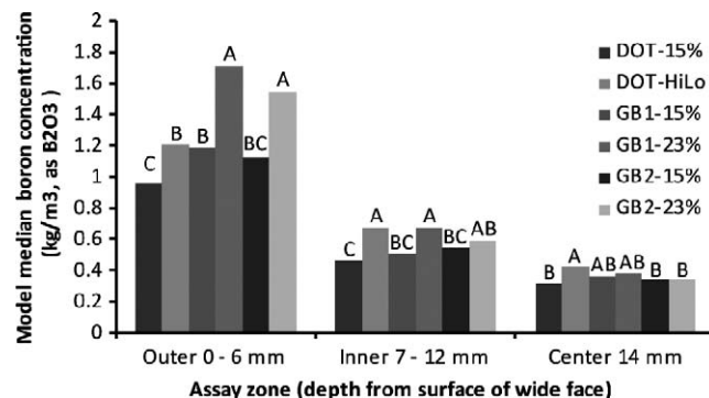
Figure 2.—Pairwise comparison of median boron concentration (expressed as kilograms per cubic meter B_2O_3 ) in each assay zone. Because the data have a lognormal distribution, statistical comparisons were performed on medians instead of means. Medians within a common assay zone and having the same letter are not significantly different at the 0.05 significance level.
