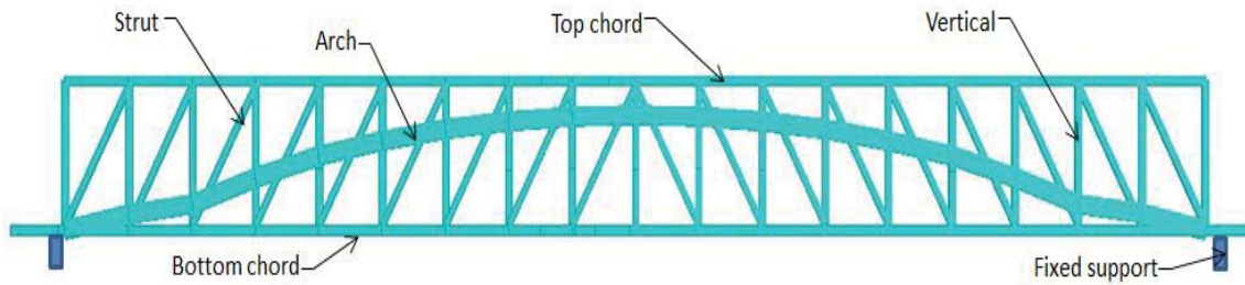
Fig. 8 STAAD model of the Cox Ford Bridge
