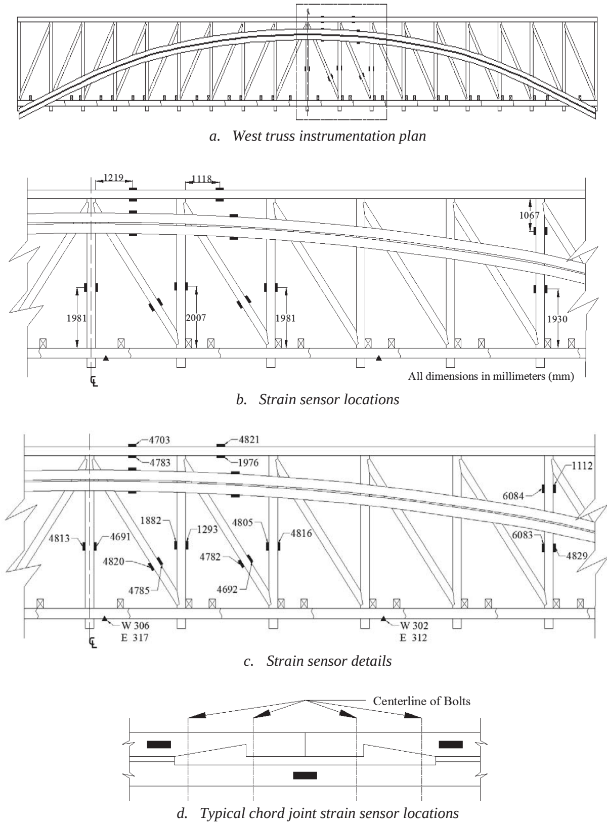
Fig. 2 Strain sensor locations for the Cox Ford Bridge load testing
