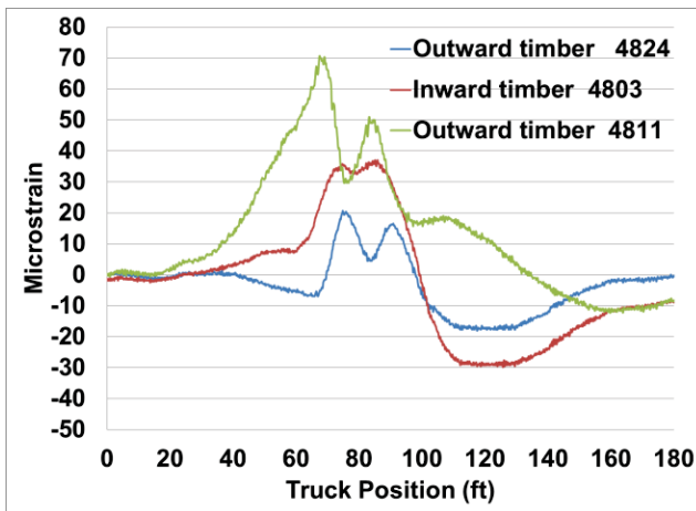
Fig. 7 East Truss Bottom of Bottom Chord, LC3
