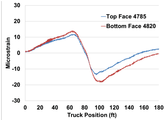
Fig. 6 West Truss Diagonal Between 9W and 10 W, LC1
