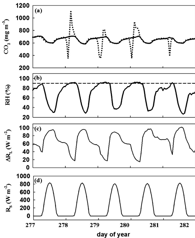
Fig. 13. Panel (a) shows the time series of \text{CO}_2 concentration measured with the EC155 (solid line) and the LI-7500 (dotted line) from DOY 277–DOY 282, 2011. Relative humidity (RH) is shown in panel (b), the difference between outgoing and incident long-wave radiation ( \Delta R_L ) is shown in (c), and incident shortwave radiation ( R_s ) is shown in (d). No precipitation was recorded on these days. The horizontal dashed line in panel (b) indicates 90% RH.
