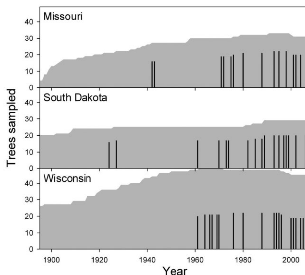
Figure 1. Number of trees sampled for each of three collection regions for ring widths (grey area) and the selected years sampled for \delta^{13}\text{C} (histogram).
