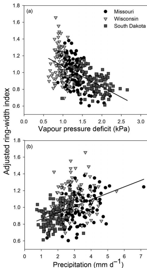
Figure 4. Adjusted ring-width index (RWI a ) plotted versus growing season vapour pressure deficit (VPD) (a) and precipitation (b).
