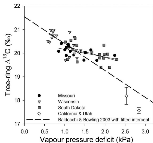
Figure 7. Tree-ring \Delta^{13}\text{C} versus vapour pressure deficit (VPD) is shown by symbols across years for Missouri (MO), Wisconsin (WI) and South Dakota (SD). The symbols for California (CA) and Utah (UT) are means among trees ( \pm 1 SE). The dashed line is the canopy-level response (see Fig. 6a) with intercept fitted to the tree-ring \Delta^{13}\text{C} data.
