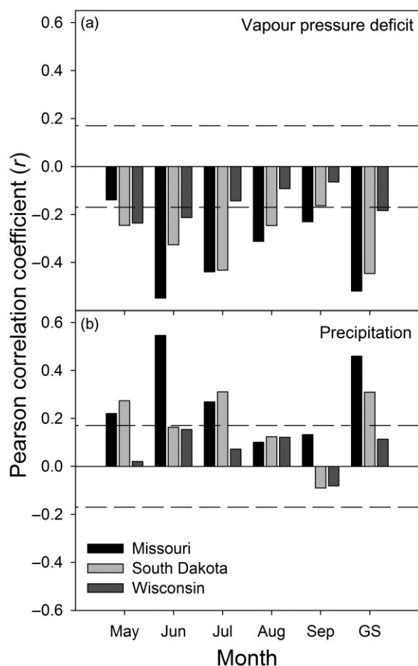
Figure 3. Correlations between ring-width indices (RWIs) and vapour pressure deficit (VPD) (a). Correlations between RWI and precipitation (b). The growing season average values are denoted as GS. The dashed lines indicate approximately where the 95% significance level occurs for a Gaussian white noise process ( n = 113 ).
