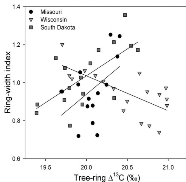
Figure 9. Ring-width index values versus tree-ring \Delta^{13}\text{C} of bur oaks growing in three regions.
