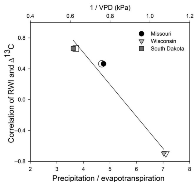
Figure 10. Correlations of ring-width indices and tree-ring \Delta^{13}\text{C} from each region scale with either of the ratio of precipitation to evapotranspiration (filled symbols) or 1/\text{VPD} (open symbols). Across this wetness gradient the trend line and labels indicate a continuum of changes in the relative influence of irradiance and moisture in limiting photosynthetic carbon gain and tree-ring growth.
