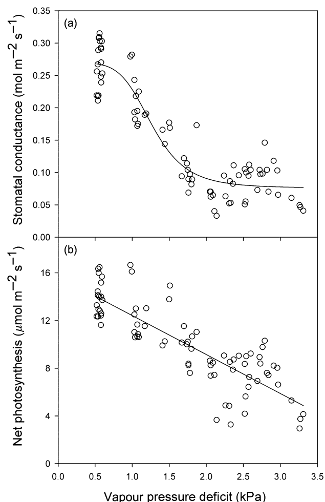
Figure 5. Gas exchange measurements made on leaves of bur oaks show vapour pressure deficit responses of stomatal conductance (a) and net photosynthesis (b). The least squares regression line fitted to stomatal conductance values was a four-parameter logistic relationship. Net photosynthesis was plotted for a leaf external [\text{CO}_2] equal to 350 ppm and saturating photon flux density (PFD).
