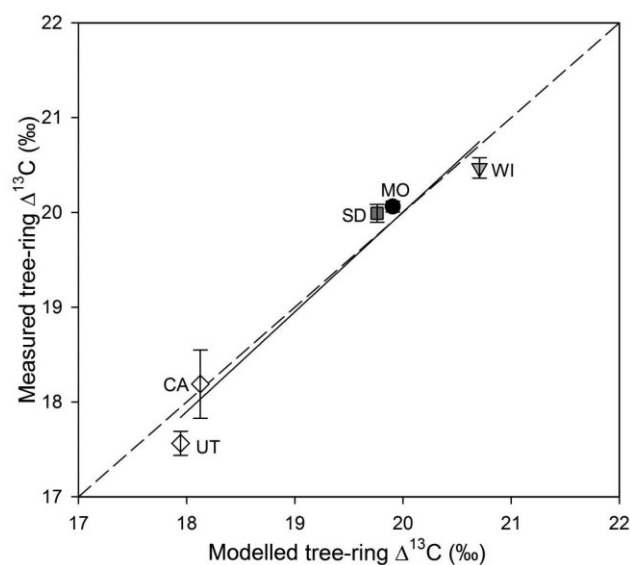
Figure 8. Comparison of modelled and observed tree-ring \Delta^{13}\text{C} ( \pm 1 SE) by region using growing season vapour pressure deficit (VPD) and photon flux density (PFD). The least squares linear relationship ( R^2 = 0.96 , P = 0.003 ) was not significantly different from the dashed 1:1 line ( P = 0.693 ). \Delta^{13}\text{C} was modelled using an equation that combined the responses of canopy-level \Delta^{13}\text{C} to VPD and PFD (see the Methods and Results sections).
