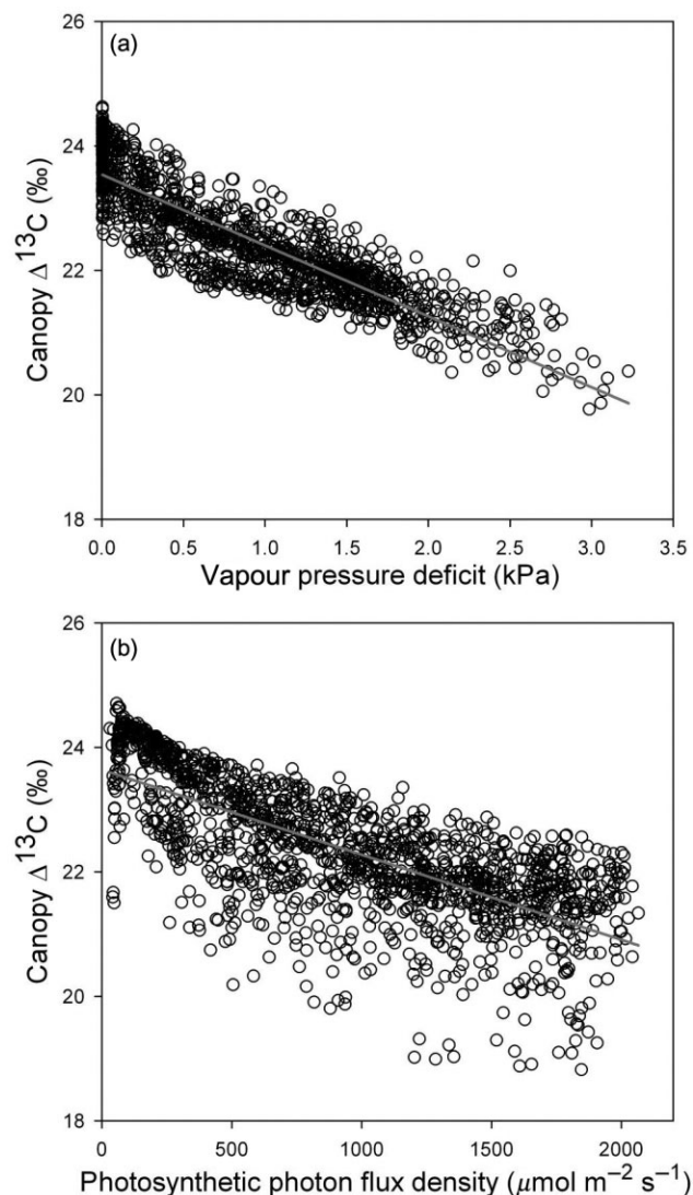
Figure 6. Canopy-integrated \Delta^{13}\text{C} estimated by the CANISOTOPE model versus vapour pressure deficit (a) and photosynthetic photon flux density (b) after Baldocchi & Bowling (2003).
