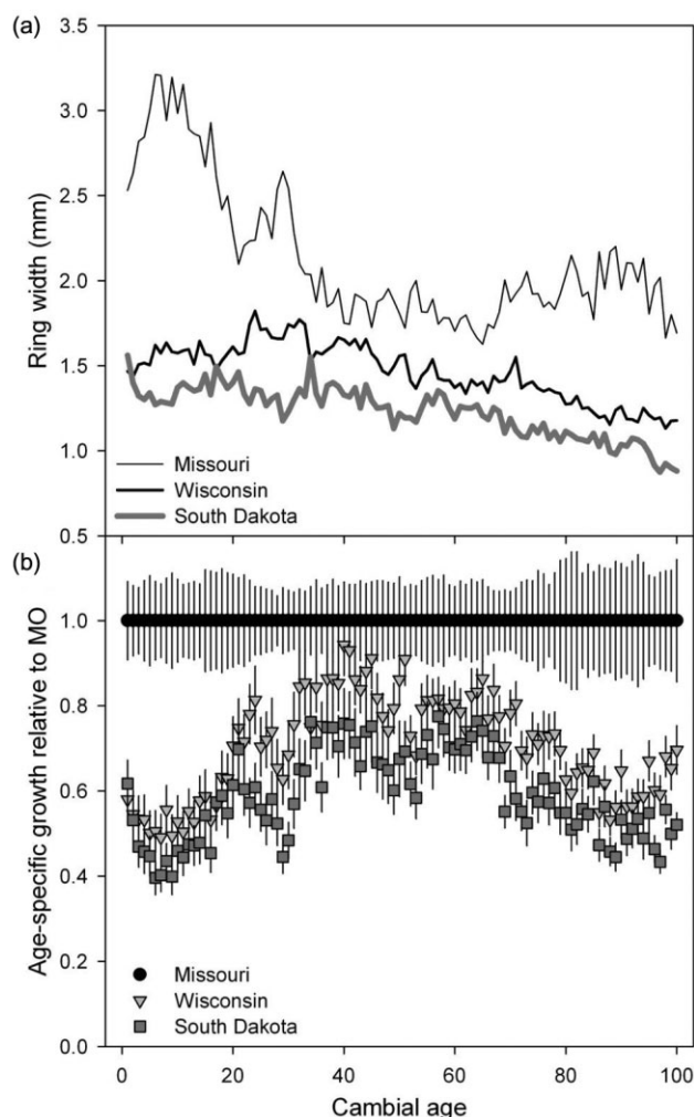
Figure 2. Mean ring widths for each region plotted by cambial age (a). Patterns in mean age-specific growth ( ASG_r ), see the Materials and Method sections) plotted by cambial age (b). Error bars are ( \pm 1 SE among trees).
