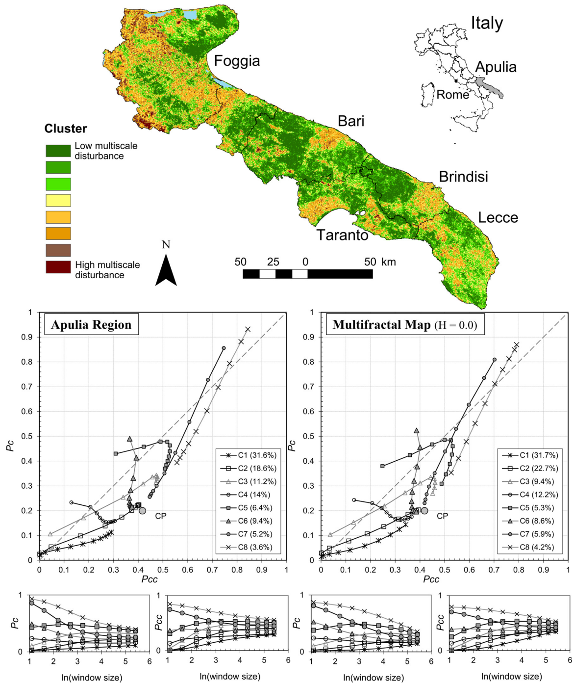
Fig. 5. Example of cross-scale cluster profiles in the Apulia region and their geographical representation ( P_c and P_{cc} refer to disturbance; modified after Zurlini et al., 2007; Zaccarelli et al., 2008). Real (left) and simulated multifractal (right) profiles. Percentages refer to the number of pixels for each cluster profile (C) with respect to all pixels of the entire region.
