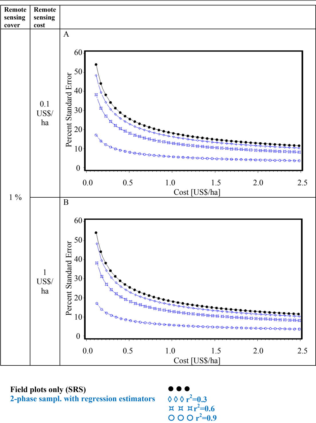
Figure 2 Sampling design alternatives, field assessment cost: 5, 000 US$ per field plot, and remote sensing cover of 1%.
