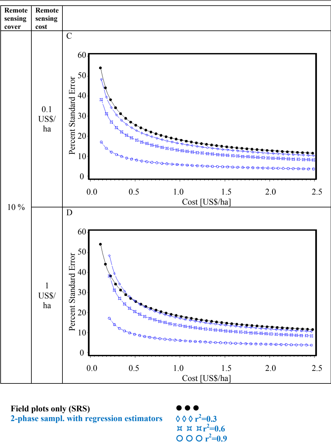
Figure 3 Sampling design alternatives, field assessment cost: 5, 000 US$ per field plot, and remote sensing cover of 10%.
