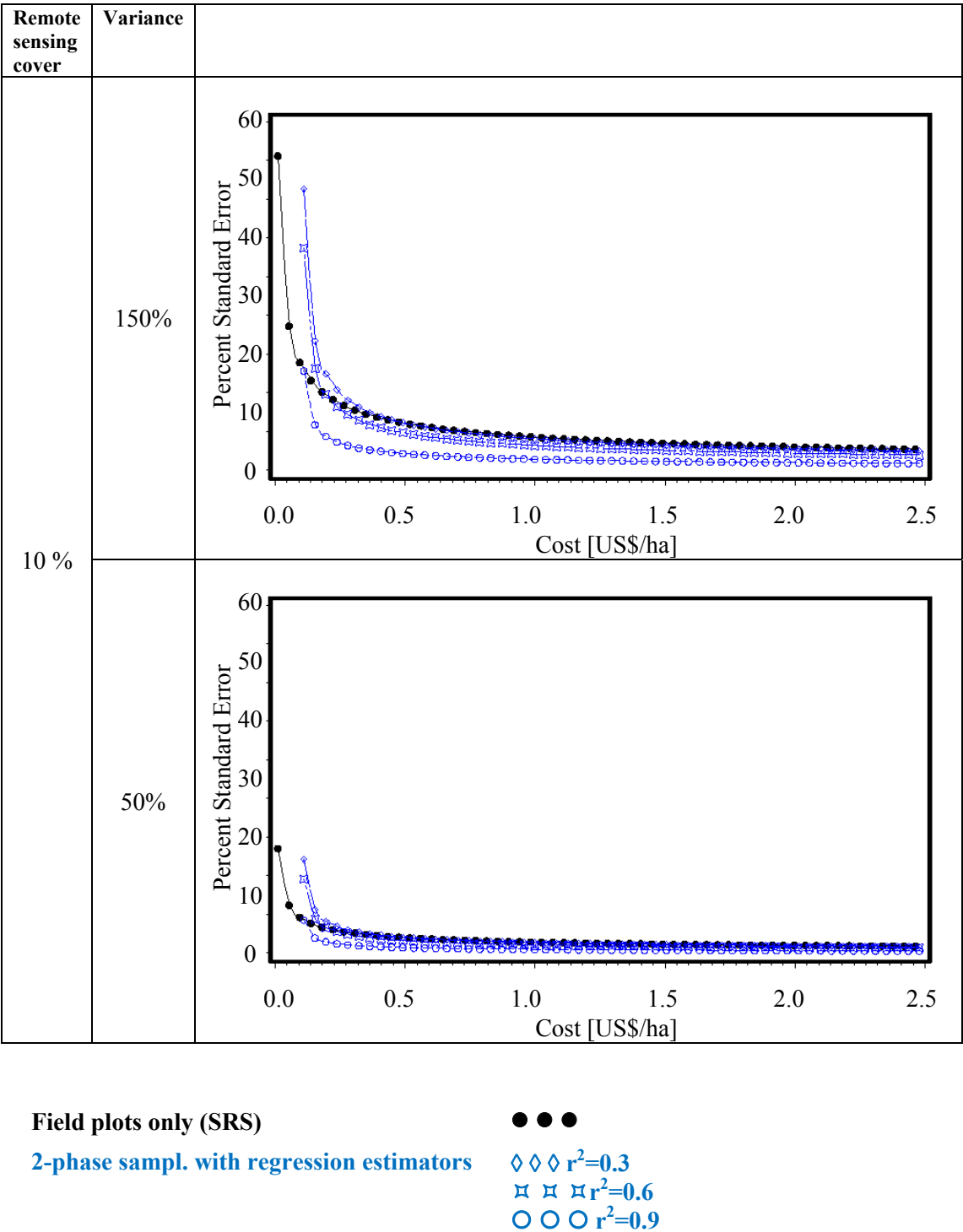
Figure 9 Cost-efficiency under changing population variances (cost per field plot = 500 US$), and remote sensing cover of 10%.
