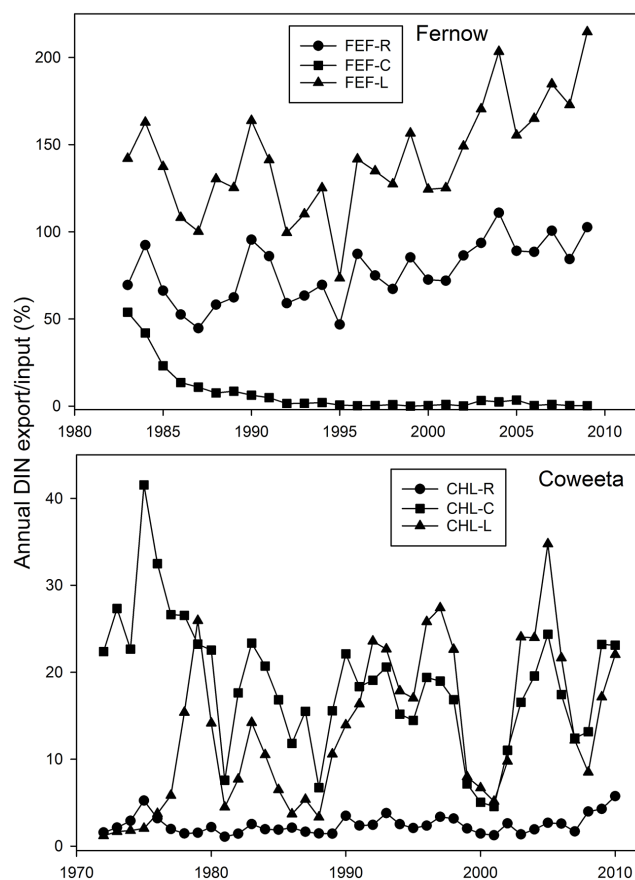
Fig. 7. Ratio of annual dissolved inorganic N (DIN) export to input for the six watersheds at the Fernow Experimental Forest (top) and Coweeta Hydrologic Laboratory (bottom).
