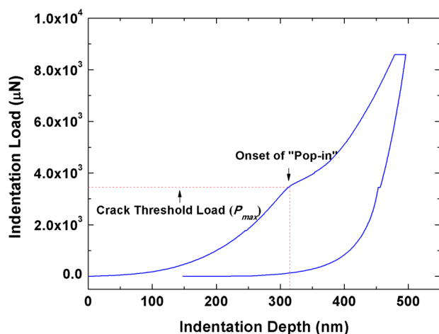
FIG. 2. (Color online) Representative pop-in identified in the loading segment of the SiCOH load-depth trace. The data comes from test on a 500 nm water-saturated UV-cured SiCOH film after conditioning at 10% RH. Reprinted with permission from Guo et al. , J. Appl. Phys. 114 , 084103 (2013). Copyright 2013, American Institute of Physics.
