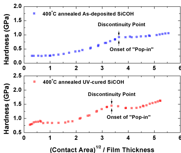
FIG. 3. (Color online) Hardness ( H ) of SiCOH films as a function of \sqrt{A_c}/h_f , where A_c is the contact area and h_f is the film thickness. The data comes from measurements on 400 °C annealed as-deposited and UV-cured SiCOH after conditioning at 10% RH. Reprinted with permission from Guo et al. , J. Appl. Phys. 114 , 084103 (2013). Copyright 2013, American Institute of Physics.
