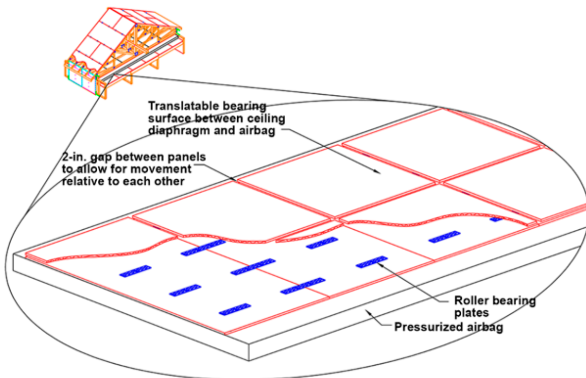
Figure 9. Specimen uplift and lateral load apparatus.
