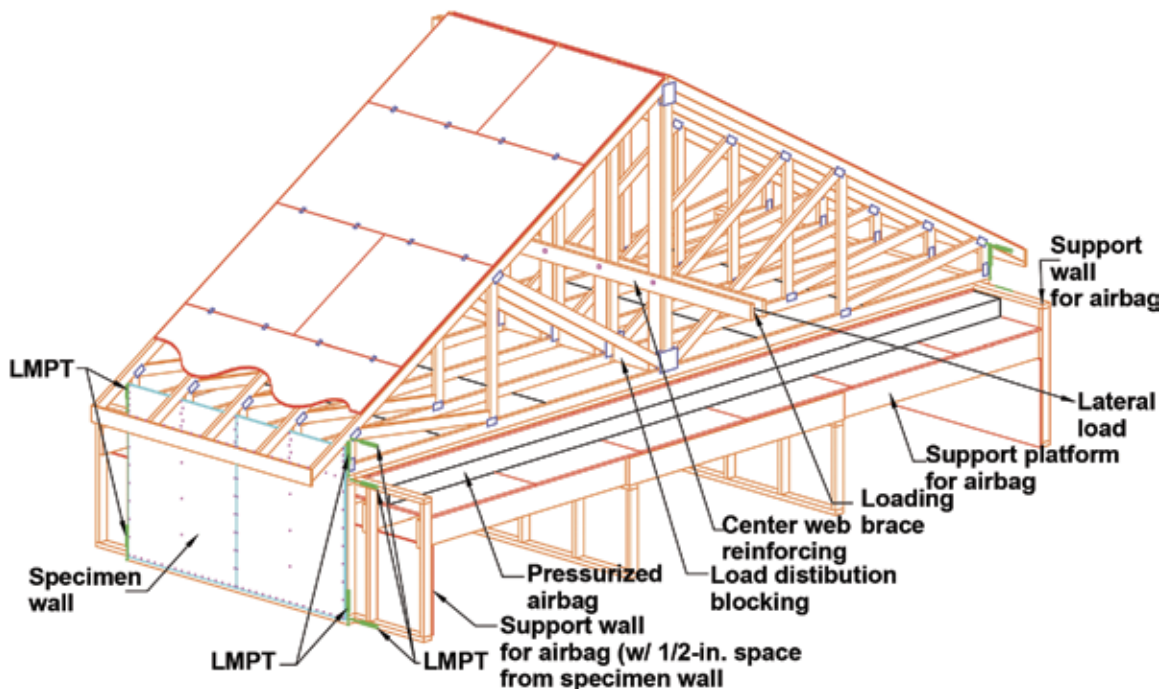
Figure 7. Test setup and instrumentation (LMPT is linear motion position transducers).
