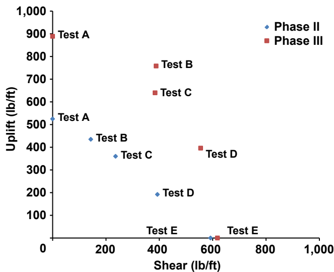
Figure 15. Comparison of Phase II and Phase III results.
