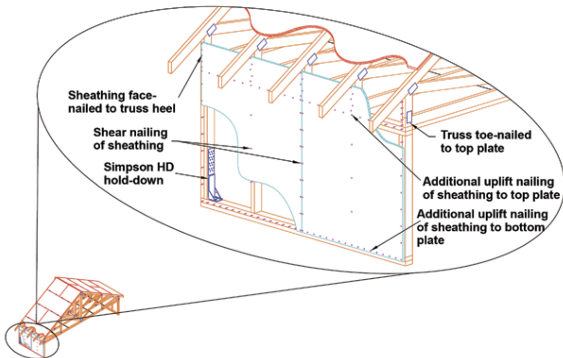
Figure 3. OSB sheathing connection detail.
