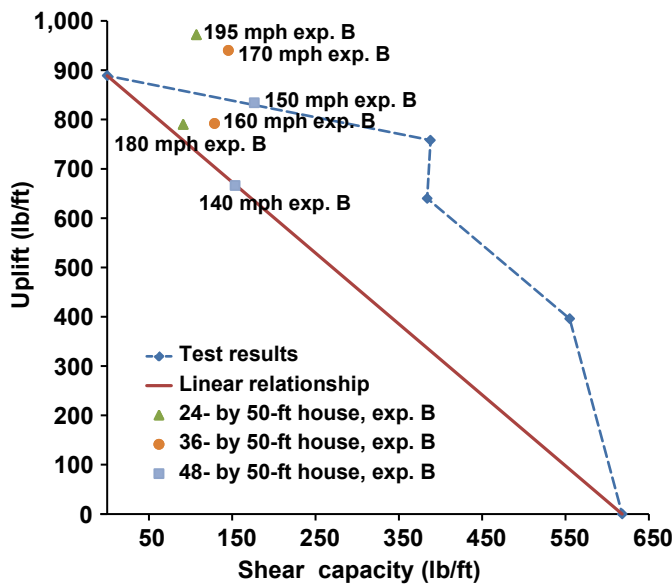
Figure 16. Comparison of tested capacity to typical wind loading scenarios (Exposure B regions).
