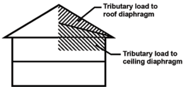
Figure 6. Tributary area of wind loads.
