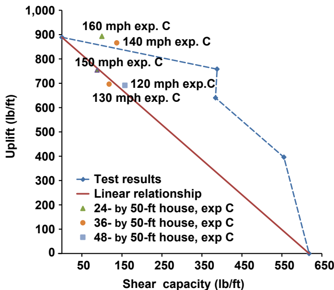
Figure 17. Comparison of tested capacity to typical wind loading scenarios (Exposure C regions).
