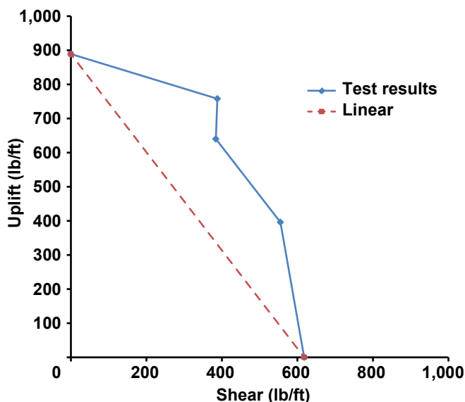
Figure 10. Uplift versus shear interaction curve from testing.
