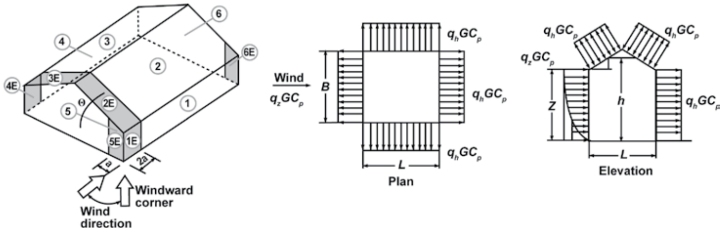
Figure 5. ASCE 7-10 wind loading profile.
