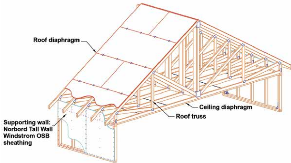
Figure 2. Specimen construction.
