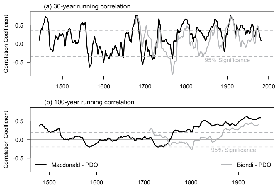
Figure 6. Running correlation analysis for (a) 30 years and (b) 100 years between GSL level and two PDO reconstructions (Biondi et al., 2001; MacDonald and Case, 2005). GSL: Great Salt Lake; PDO: Pacific Decadal Oscillation.
