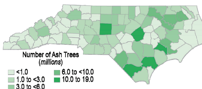
Figure 2—Population of ash trees \geq 1 inch d.b.h. by county.
