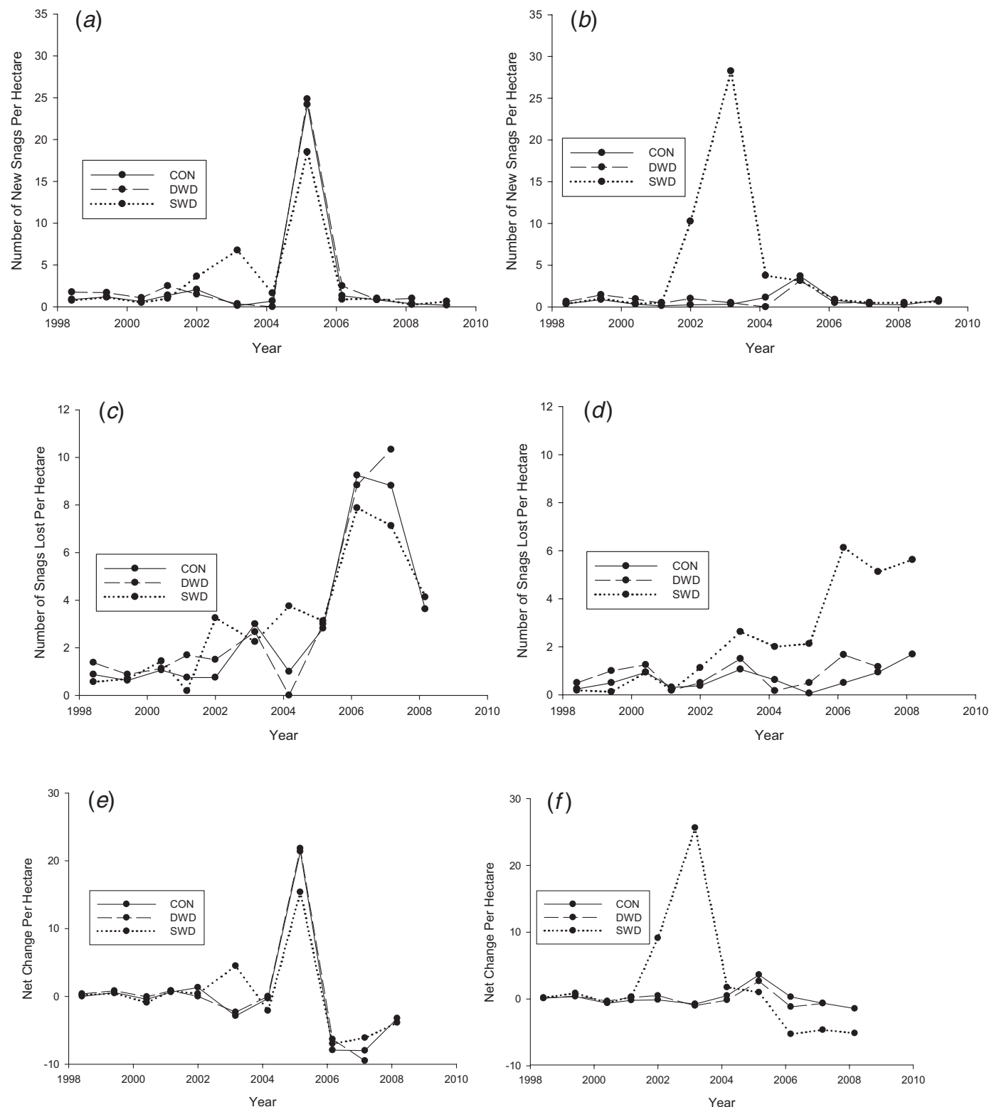
Fig. 3. The rates of recruitment ( a and b ), loss ( c and d ), and net change ( e and f ) for small (<25 cm DBH) and large ( \geq 25 cm DBH) size snags, respectively, for the control (CON), down woody debris (DWD), and standing woody debris (SWD) treatments during the pretreatment (1996–2001) and post-treatment (2001.9–2009) periods. Net change is defined as recruitment minus loss.
