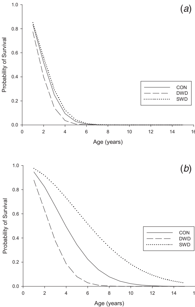
Fig. 4. Modeled probability of snag survival as a function of snag age (years since tree death) for small (<25 cm DBH) (a) and large (≥25 cm DBH) (b) size snags for the control (CON), down woody debris (DWD), and standing woody debris (SWD) treatments during the post-treatment (2001.9–2009) period.
