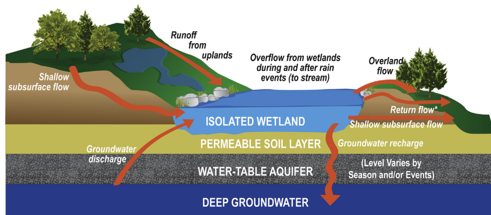
Fig. 2. Conceptual model of how GIWs are connected hydrologically to surface water systems where a permeable soil layer exists beneath the GIW (i.e., multi-directional flow systems).
