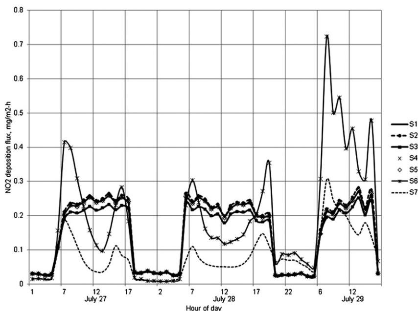
Fig. 5. Time-series comparison of modeled NO 2 hourly deposition fluxes averaged over all grid cells.
