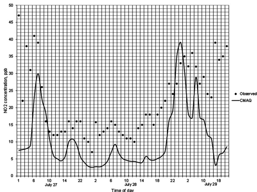
Fig. 7. Time-series comparison of measured and modeled surface-level \text{NO}_2 concentration, in ppb, from July 27 to 29, 2005 measured at the downtown Baltimore monitoring station.
