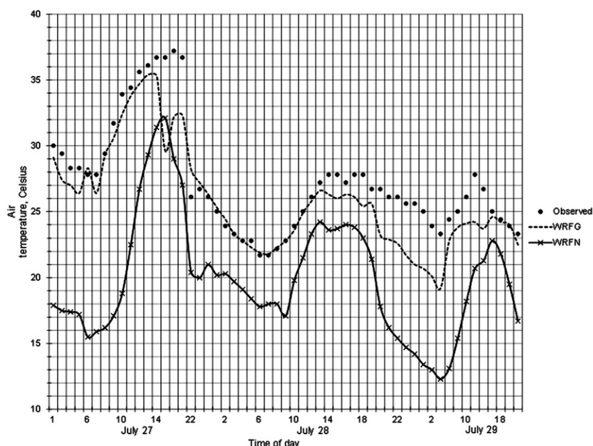
Fig. 6. Time-series comparison of measured and modeled near-surface temperature, in °C, from July 27 to 29, 2005 measured at the monitoring station in Baltimore.
