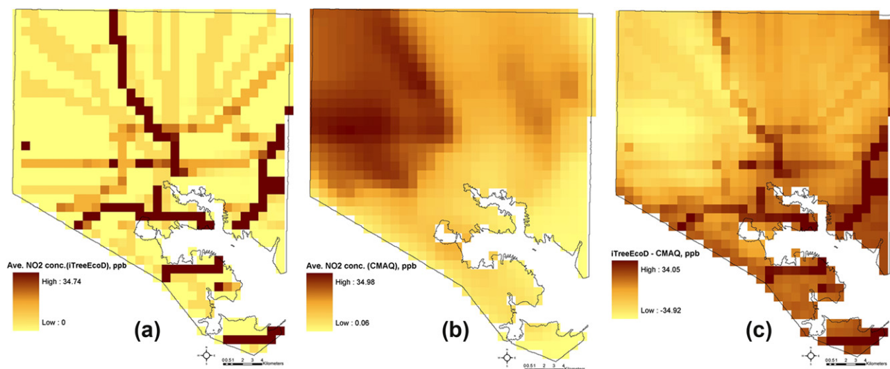
Fig. 4. Spatial plots of time-averaged (a) iTreeEcoD- (S1, S2, S3, S4, and S5) and (b) CMAQ-modeled (S6 and S7) NO 2 concentration (ppb), and (c) the differences in these concentrations for Baltimore, MD.
