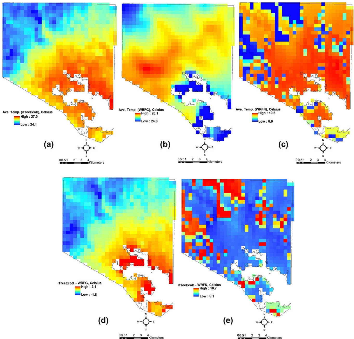
Fig. 3. Spatial plots of time-averaged 2-m temperatures (°C) modeled by the (a) iTreeEcoD (S1, S2, S3, and S6), (b) WRFG (S4 and S7), and (c) WRFN (S5); and differences between iTreeEcoD- and (d) WRFG- and (e) WRFN-modeled 2-m air temperatures for Baltimore, MD.
