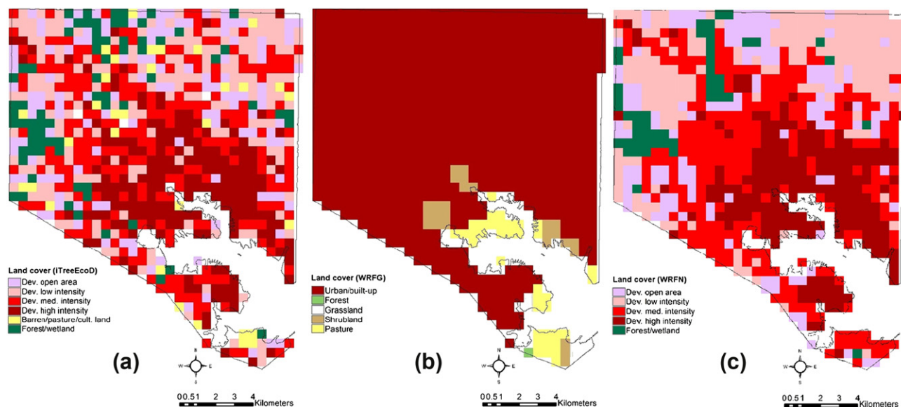
Fig. 2. Land cover data (a) obtained from NLCD 2001 (S1, S4, S5, and S6); (b) extracted from WRF using GLCC (S2 and S7); and (c) extracted from WRF using NLCD (S3).
