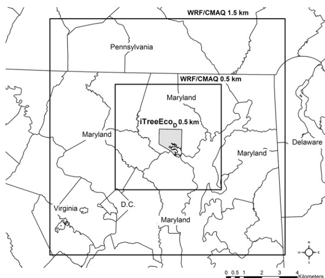
Fig. 1. Modeling domain showing locations of the WRF, CMAQ, and iTreeEco D grids.
