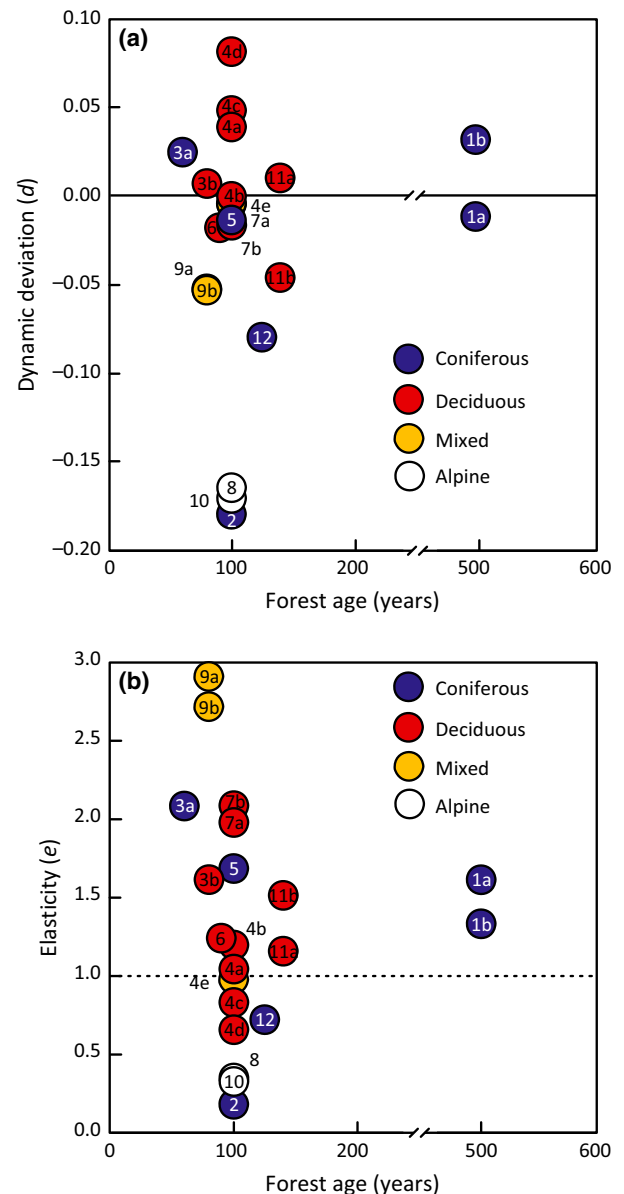
Fig. 8 Catchment properties as a function of forest type (colored circles) and forest age: (a) dynamic deviation d and (b) elasticity e . Key to site IDs (the numbers within the circles) is given in Table 1. (Color in the online version)
