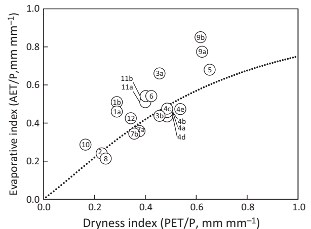
Fig. 4 Mean annual dryness index and evaporative index values for headwater catchments during the 5-water-year cool period. The dotted line represents the Zhang et al. (2001) modification of the Budyko curve ( w = 2 ). The vertical displacement of each point from the Budyko curve is the static deviation s . Key to site IDs (the numbers within the circles) is given in Table 1.
