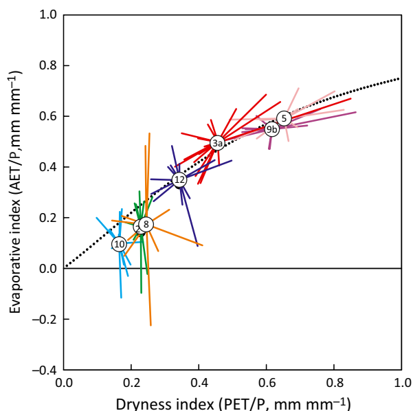
Fig. 6 Year-to-year variability in mean annual dryness index and evaporative index values for selected headwater catchments during period of record with static deviation ( s ) removed from each value. The numbered circles represent the mean annual values over the period of record. The radiating lines indicate annual excursions from that mean. The longer the line, the greater the departure from the long-term mean value. The dotted line represents the Zhang et al. (2001) modification of the Budyko framework ( w = 2 ). Key to site IDs (the numbers within the circles) is given in Table 1.
