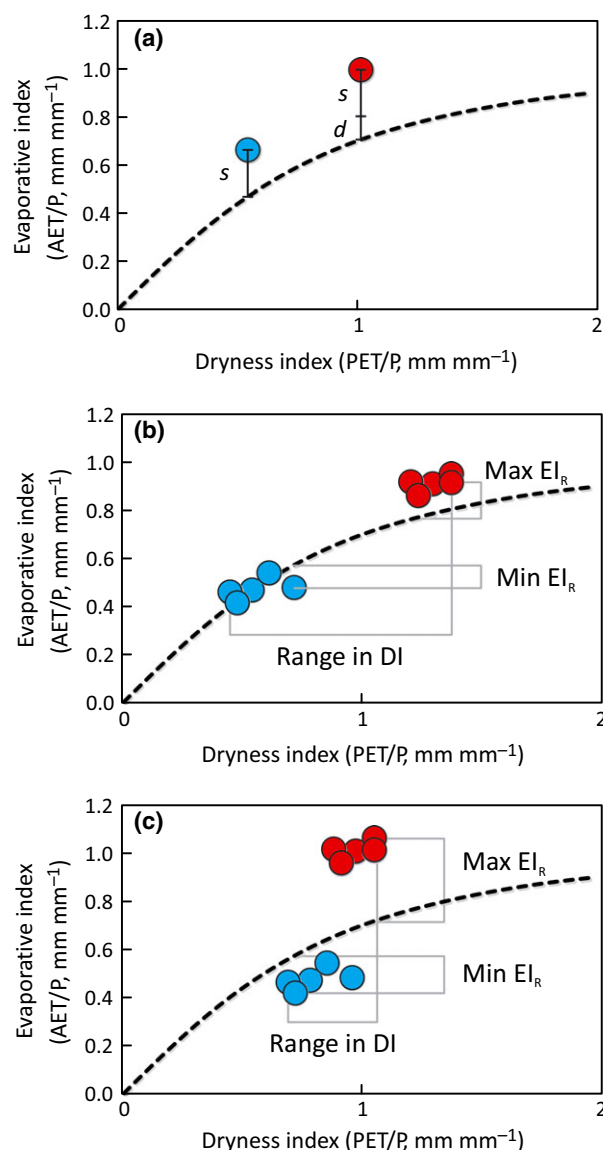
Fig. 3 Graphical representation of Budyko resilience metrics. Each dot shows a catchment's paired dryness index (DI) and evaporative index (EI) values: blue for the cool period and red for the later warm period. The dashed line represents the theoretical Budyko curve. (a) Static deviation ( s ) was calculated as the difference between measurement-based and theoretical evaporative indices during the catchment's cool period: s = EI_{M,cool} - EI_{B,cool} . Dynamic deviation ( d ) was calculated as the analogous warm-period quantity, corrected for the previously determined s : d = EI_{M,warm} - EI_{B,warm} - s . Points that fall above the theoretical curve indicate smaller-than-predicted water yields; points that fall below the curve indicate larger-than-predicted yields. Elasticity ( e ) was calculated as the ratio of a catchment's range in DI to its range in EI during the two contrasting climate periods: e = (DI_{max} - DI_{min}) / (EI_{R,max} - EI_{R,min}) . (b) This example catchment exhibited a high degree of elasticity ( e > 1 ) (i.e., approximating theoretical behavior). (c) This example catchment exhibited low elasticity ( e < 1 ) (i.e., deviating from theoretical behavior).
