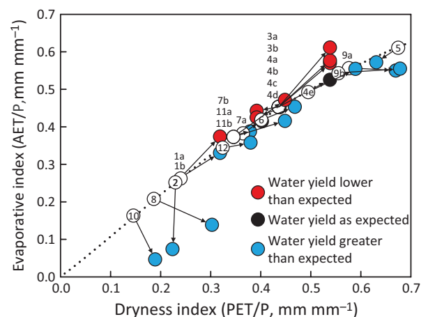
Fig. 5 Mean cool-period and warm-period dryness index (DI) and evaporative index (EI) values for headwater catchments showing catchment transitions from 5-water-year (5-wyr) cool period (numbered circles) to 5-wyr warm period (colored circles) with static deviation ( s ) removed from both periods. Arrows denote the direction of movement from cool to warm period. Red circles denote catchments with decreases in expected water yield (increasing EI); blue circles denote catchments with increases in expected water yield (decreasing EI); and black circles denote catchments with expected water yield. The dotted line represents the Zhang et al. (2001) modification of the Budyko framework ( w = 2 ). Key to site IDs (the numbers within the circles) is given in Table 1. (Color in the online version)
