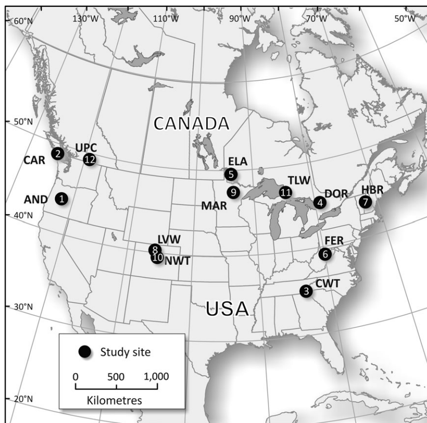
Fig. 2 Location of long-term monitoring catchments that met the selection criteria for this study ( n = 12 ). Site identifiers are: 1, HJ Andrews; 2, Carnation; 3, Coweeta; 4, Dorset; 5, Experimental Lakes Area; 6, Fernow; 7, Hubbard Brook; 8, Loch Vale Watershed; 9, Marcell; 10, Niwot; 11, Turkey Lakes Watershed; 12, Upper Penticton.
