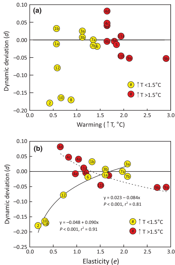
Fig. 7 Dynamic deviations of headwater catchments as a function of (a) warming and (b) elasticity. The color of the circle represents the extent of warming over the cool-to-warm transition (yellow = <1.5 °C warming; red = >1.5 °C warming). The long-dash line in (b) represents the relationship between d and e for catchments that experienced <1.5 °C warming. The short-dash line in (b) represents the relationship between d and e for catchments that experienced >1.5 °C warming. Key to site IDs (the numbers within the circles) is given in Table 1.
