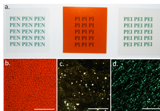
Figure 2. (a) Photograph of polyetherimide (PEI), polyimide (PI), and polyethylene naphthalate (PEN) \sim 5 \text{ cm} \times 5 \text{ cm} films. (b) BF image of a PI film. (c) PC image of a PEN film. (d) PL image of a PEI film. Scale bar 500 \mu\text{m} . Textures observed for PEI, PI, and PEN films under all microscopy modes are available in Figure S1 in Supporting Information.
