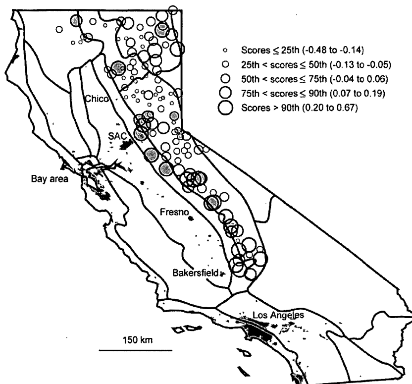
Figure 7. Map of air scores. Circles represent lichen community plots. Classes are based upon the 25th, 50th, 75th, and 90th percentiles of air scores at on-frame plots. Off-frame plots and urban areas are shaded gray. SAC = Sacramento.
