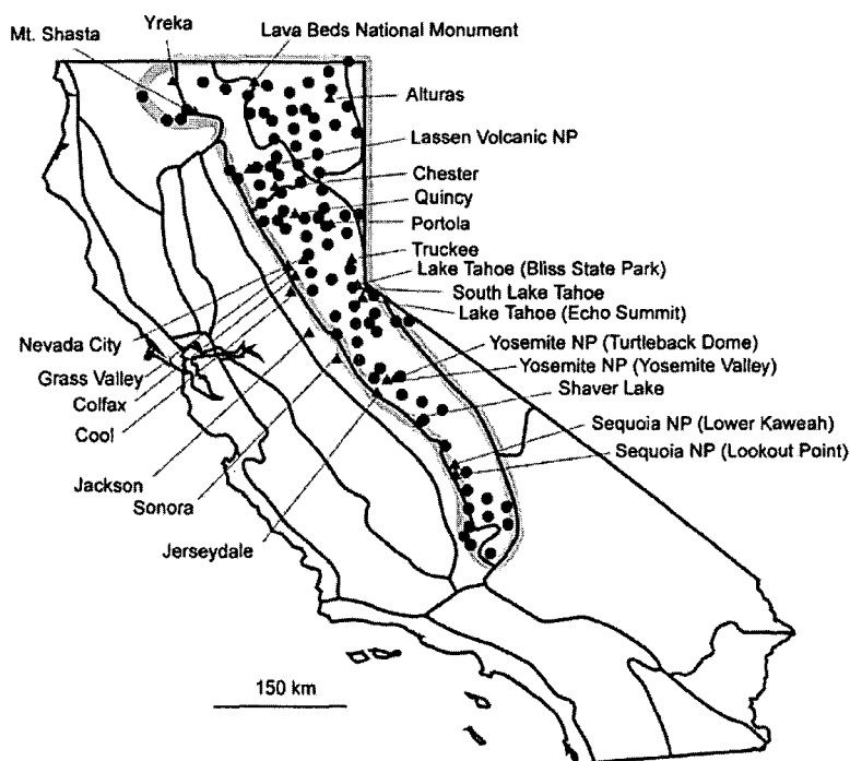
Figure 1. Map of greater Sierra Nevada model area. Model boundary is delineated by thick gray line. Thinner black lines indicate Bailey's ecoregions (Bailey 1983). Triangles indicate off-frame plots while circles indicate on-frame plots. NP = National Park.
