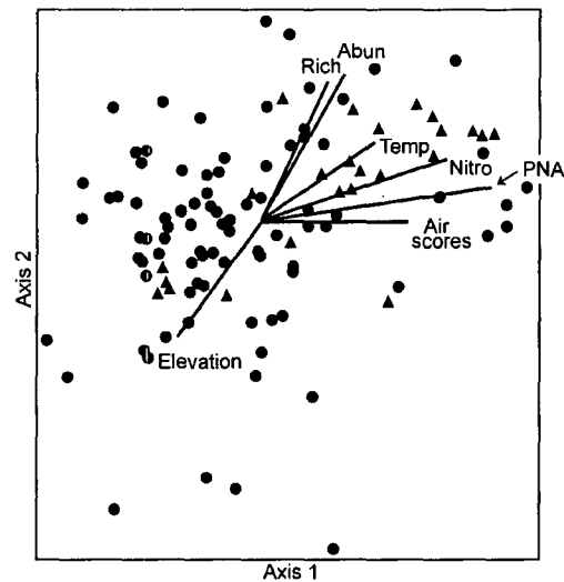
Figure 2. Ordination joint plot with environmental and lichen community variables overlaid. Triangles indicate off-frame plots while circles indicate on-frame plots. Vector lengths and directions indicate correlations with the ordination. Most vectors with r^2 > 0.25 are shown. To prevent crowding, related variables with overlapping vectors of similar strength are designated by a single label: Temp (temperature) represents dew temperature, mean temperature, minimum temperature, and maximum temperature; Nitro includes nitrophyte diversity and abundance; and PNA includes proportion of species richness and lichen abundance at a plot in nitrophytes. Abbreviations for other environmental vectors are: Rich = total lichen species richness, Abun = total lichen abundance (sum of abundance codes), and Air scores = air quality scores adjusted for elevation.
