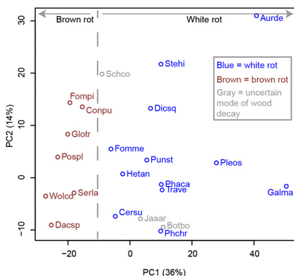
Fig. 2. Wood-decaying basidiomycetes plotted on the first two principal components from phylogenetic PCA of CAZymes (including lignin-related auxiliary activities) of the organisms.
