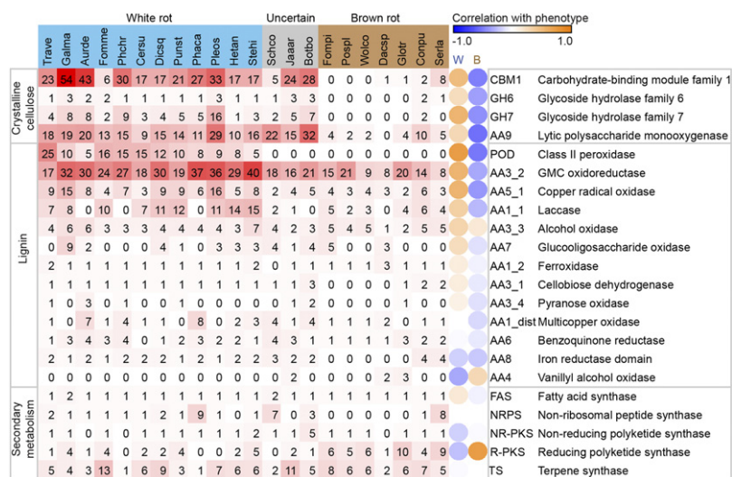
Fig. 1. Lignocellulose-degrading and secondary metabolism in wood-decaying fungi. Organisms use the following abbreviations: Aurde, Auricularia delicata ; Botbo, Botryobasidium botryosum ; Cersu, Ceriporiopsis subvermispora ; Conpu, Coniophora puteana ; Dacsp, Dacryopinax sp.; Dicsq, Dichomitus squalens ; Fomme, Fomitopsis mediterranea ; Fompi, Fomitopsis pinicola ; Galma, Galerina marginata ; Glotr, Gloeophyllum trabeum ; Hetan, Heterobasidium annosum ; Jaar, Jaapia argillacea ; Phaca, Phanerochaete carnosae ; Phchr, Phanerochaete chrysosporium ; Pleos, Pleurotus ostreatus ; Pospl, Postia placenta ; Punst, Punctularia strigosozonata ; Schco, Schizophyllum commune ; Serla, Serpula lacrymans ; Stehi, Stereum hirsutum ; Trave, Trametes versicolor ; Wolco, Wolfiporia cocos . Gene number is shaded red/white, and independent-contrasts correlation of enzyme with rot type is shaded orange/blue. Notice a strict white/brown-rot dichotomy with respect to the lignin-attacking PODs and the CAZymes that target crystalline cellulose (CBM1, GH6, and GH7), and a continuum with other lignin-targeting enzymes.
