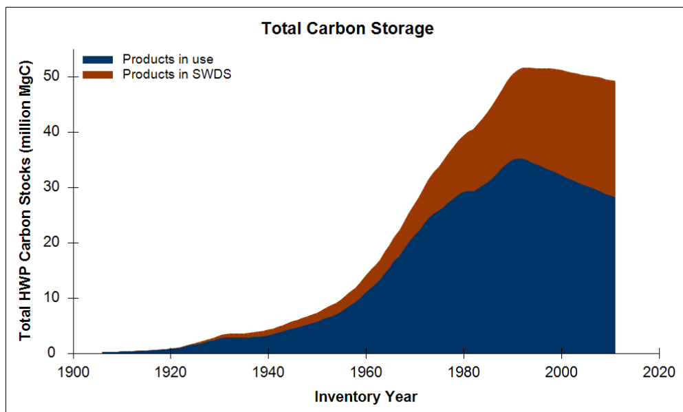
Figure 5. Cumulative total carbon stored in HWP manufactured from Pacific Southwest Region timber using the IPCC/EPA approach. Carbon in HWP includes both products that are still in use and carbon stored at solid waste disposal sites (SWDS), including landfills and dumps.
