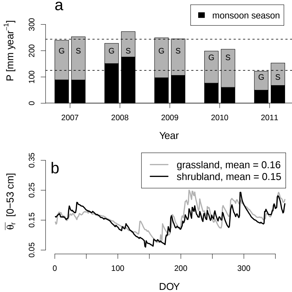
Figure 3.1: Total annual and monsoon precipitation at the creosotebush shrubland (S) and mixed grassland (G) site in 2007-2011 (Panel A) and mean daily relative extractable soil moisture [\theta_r] (Panel B). Mean monsoon precipitation and mean annual precipitation from 1996-2011 are indicated by horizontal lines in Panel A. \theta_r was greater on average at the grassland site ( p < 0.001 ).
