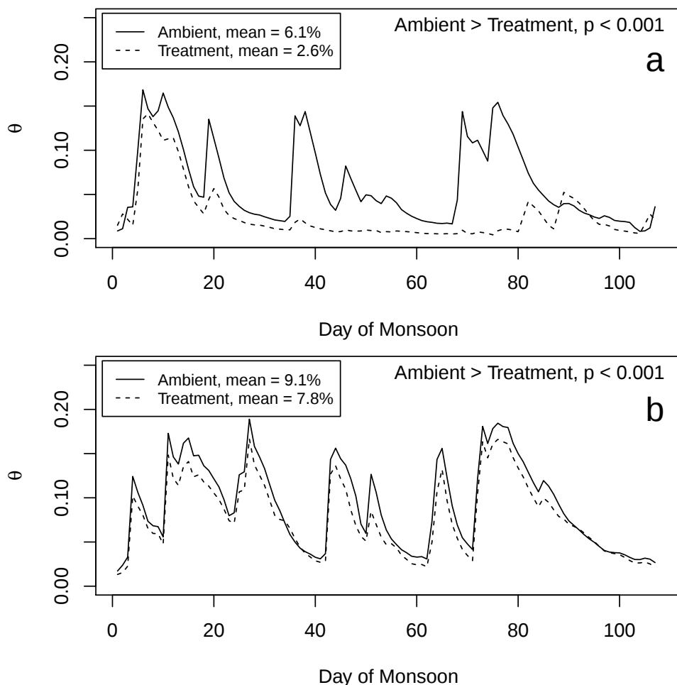
Figure 4.2: Soil moisture (0-10 cm) in ambient and treatment plots in 2012 (Panel a) and 2013 (Panel b).
