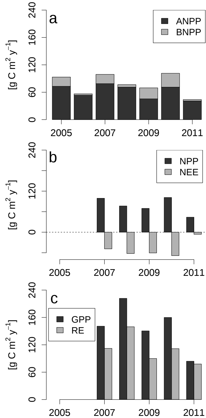
Figure 3.3: Annual aboveground [ANPP] and belowground [BNPP] production from 2005-2011 (Panel A), net primary production [NPP] and net ecosystem exchange [NEE: g m^2 y^{-1} ] from 2007-2011 (Panel B) and gross primary production [GPP] and ecosystem respiration [RE] from 2007-2011 (Panel C) in creosotebush shrubland.
