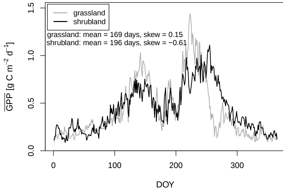
Figure 3.4: Mean daily gross primary production [GPP] from 2007-2011 shows that creosotebush shrublands have longer growing season than desert grasslands by 27 days, on average, and are notably more active late in the year.
