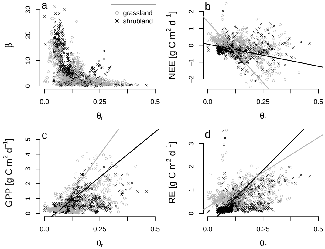
Figure 3.6: Relationship between relative extractable soil moisture [ \theta_r ] and Bowen Ratio [ \beta ] (Panel A), Net Ecosystem Exchange [NEE] (Panel B, grassland R^2 = 0.18 , shrubland R^2 = 0.01 ), Gross Primary Production [GPP] (Panel C, grassland R^2 = 0.29 , shrubland R^2 = 0.22 ) and ecosystem respiration [RE] (Panel D, grassland R^2 = 0.07 , shrubland R^2 = 0.17 ) for desert grasslands and creosotebush shrublands during their active growing seasons. All carbon flux units are in \text{g C m}^2 \text{day}^{-1} .
