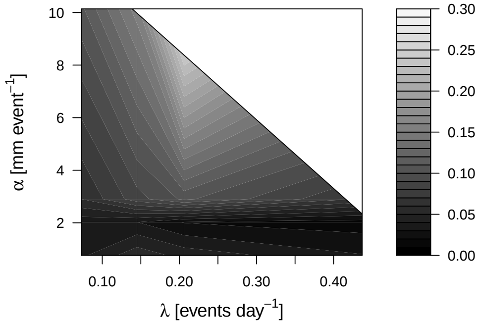
Figure 4.6: Response of daily gross primary productivity [GPP: g C m ^2 day ^{-1} ] to prior 14-day precipitation timing [ \lambda : events day ^{-1} ] and magnitude [ \alpha : mm event ^{-1} ] statistics. GPP responds strongly to \alpha , especially as \alpha increases from 2 to 3 mm event ^{-1} .
