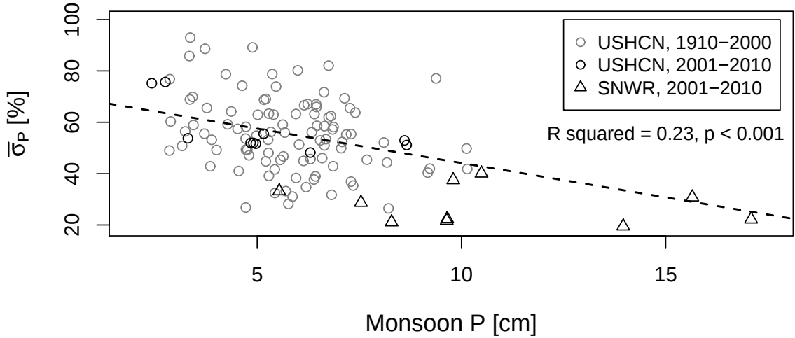
Figure 2.6: Relationship between average annual monsoon precipitation [cm] and normalized annual variability in total precipitation for USHCN sites in 1910–2010 and SNWR sensors in 2001–2010 ( R^2 = 0.23 , p < 0.001 ).
