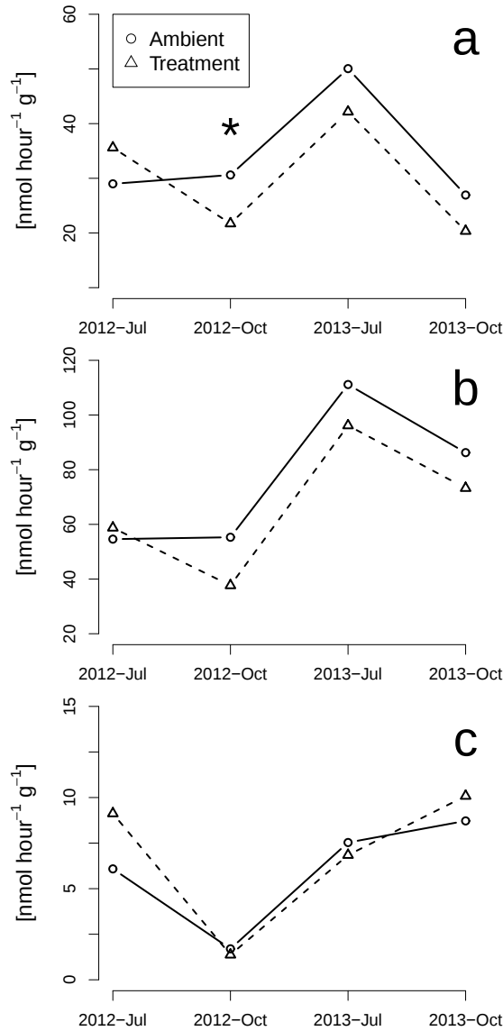
Figure 4.5: Net extracellular enzyme activity [EEA: \text{nmol hour}^{-1} \text{g soil}^{-1} ] of soil interspaces (0-10 cm depth) in ambient and treatment plots at the beginning and end of the monsoon season in 2012 and 2013. EEA data includes analysis of Alkaline phosphatase (Panel a), Alanine aminopeptidase (Panel b) and \beta -D-glucosidase (Panel c). Extracellular activity of Alkaline phosphatase was significantly higher in ambient plots at the end of the 2012 monsoon ( p < 0.05 , Panel a).
