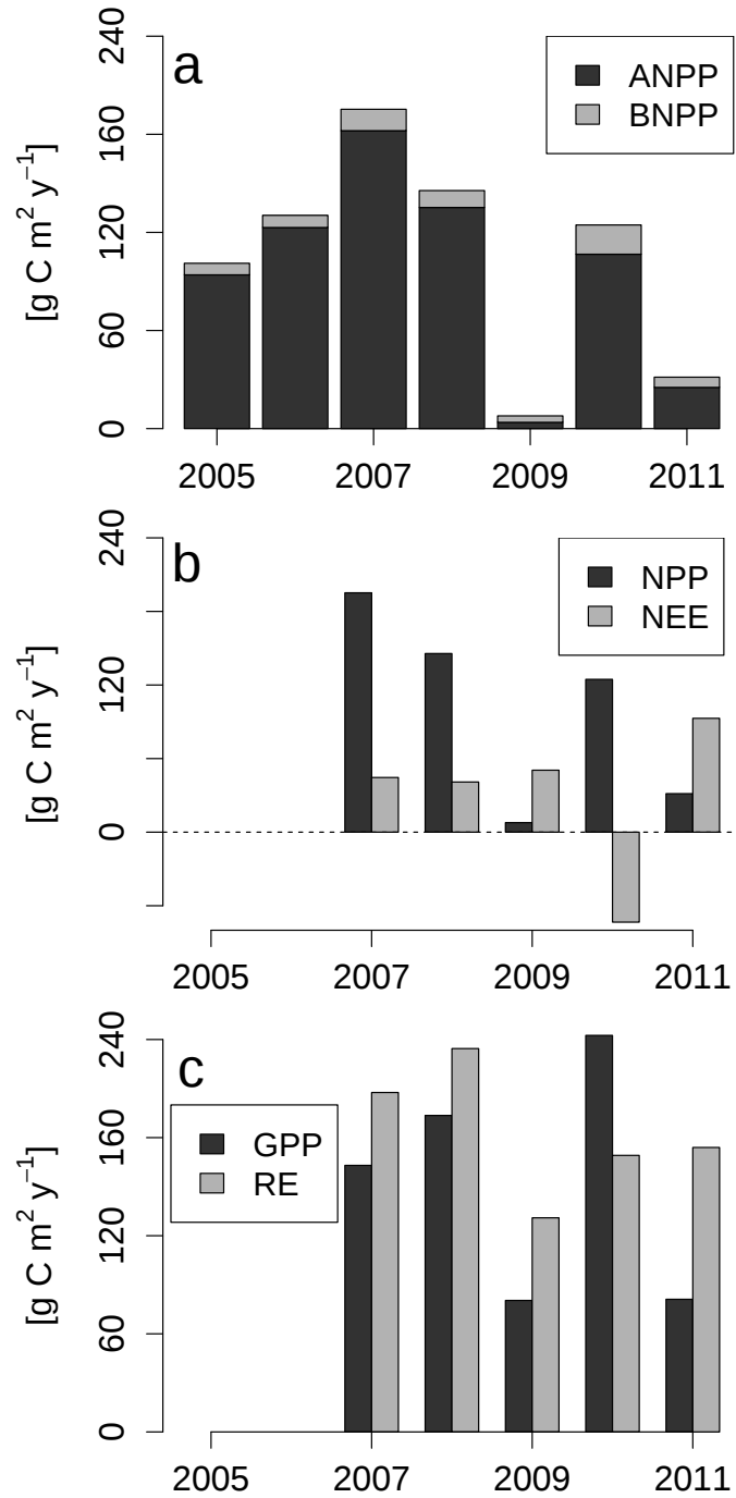
Figure 3.2: Annual aboveground [ANPP] and belowground [BNPP] production from 2005-2011 (Panel A), net primary production [NPP] and net ecosystem exchange [NEE: g m^2 y^{-1} ] from 2007-2011 (Panel B) and gross primary production [GPP] and ecosystem respiration [RE] from 2007-2011 (Panel C) in desert grassland.
