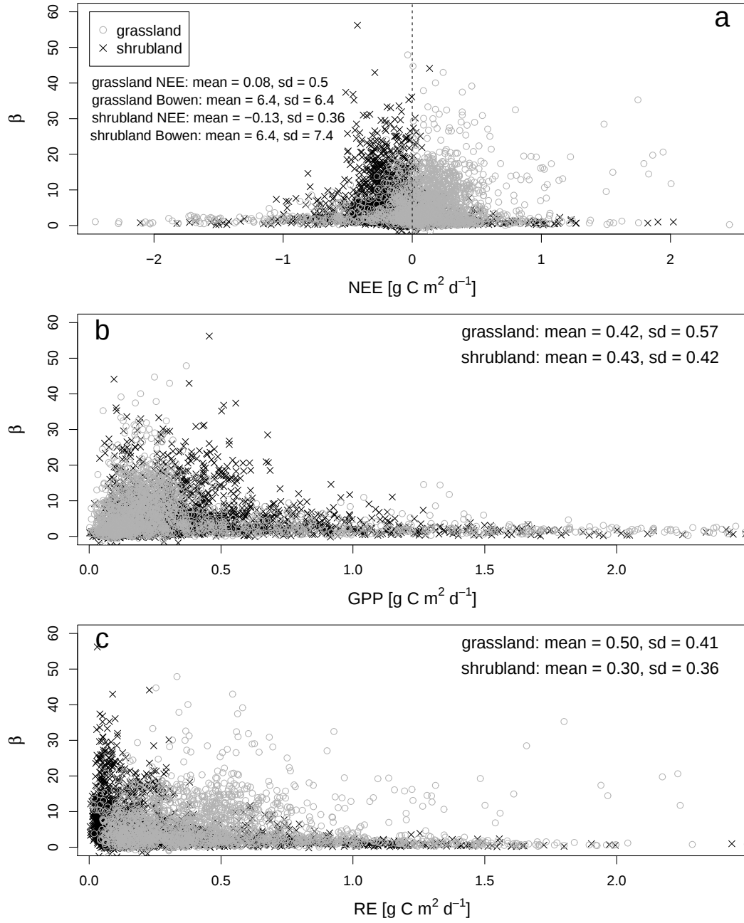
Figure 3.5: Relationship between daily Bowen Ratio [ \beta : \frac{H}{LE} ] to daily net ecosystem exchange [NEE] (Panel A), daily gross primary production [GPP] (Panel B) and daily ecosystem respiration [RE] (Panel C) in desert grasslands and creosotebush shrublands from 2007-2011. Summary statistics are included and carbon flux units are in \text{g C m}^2 \text{day}^{-1} .
