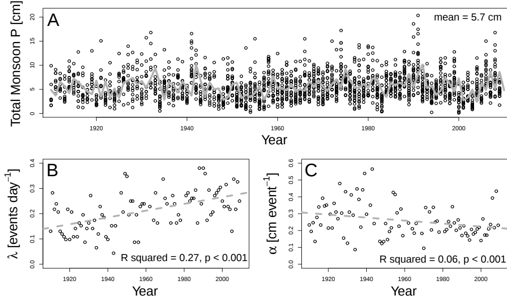
Figure 2.2: Total USHCN site precipitation (Panel A), average monsoon event timing [ \lambda : events day -1 ] (Panel B) and average monsoon event magnitude [ \alpha : depth event -1 ] (Panel C) for up to 22 sites in the northern Chihuahuan Desert from 1910-2010. Mean annual monsoon precipitation from 1910-2010 is indicated by the line in Panel A.
