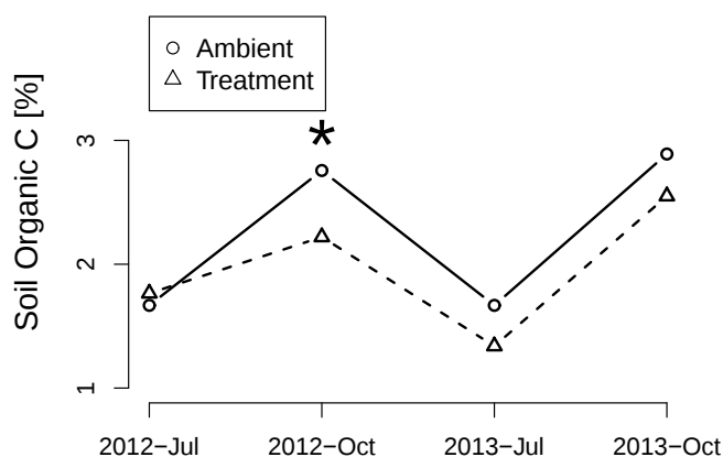
Figure 4.3: Soil organic carbon [% by mass] in ambient and treatment plots at the beginning and end of the monsoon season in 2012 and 2013. Soil C was significantly higher in ambient plots at the end of 2012 ( p < 0.03 ).
