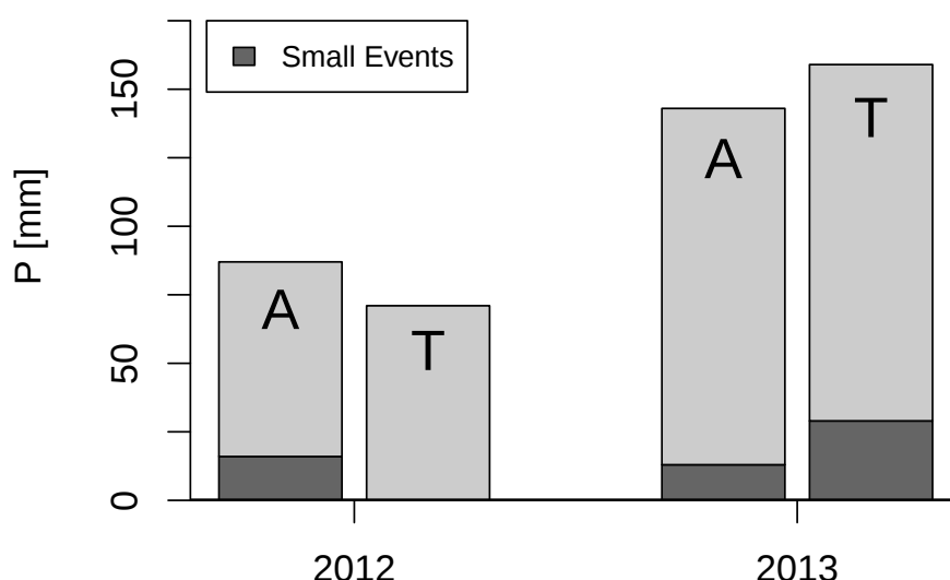
Figure 4.1: Total rainfall in ambient precipitation (A) and precipitation treatment (T) plots in 2012 and 2013. The experimental treatment in 2012 removed small rainfall events ( < 3.8 \text{ mm day}^{-1} ). In 2013, 4 small, 3.8 mm rainfall events were added incrementally to treatment plots (15.2 mm total).
