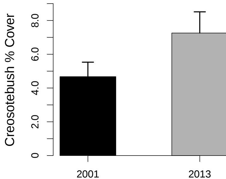
Figure 3.7: Creosotebush percent cover across two 325 m transects in creosotebush-dominated shrubland at the SNWR. Creosotebush cover [%] in 2013 was higher than in 2001 (4.7% in 2001, 7.3% in 2013, p < 0.05 ). Across two longer 1000 m transects (into blue and black grama grassland), creosotebush cover was not significantly higher in 2013 ( p > 0.13 , not shown).
