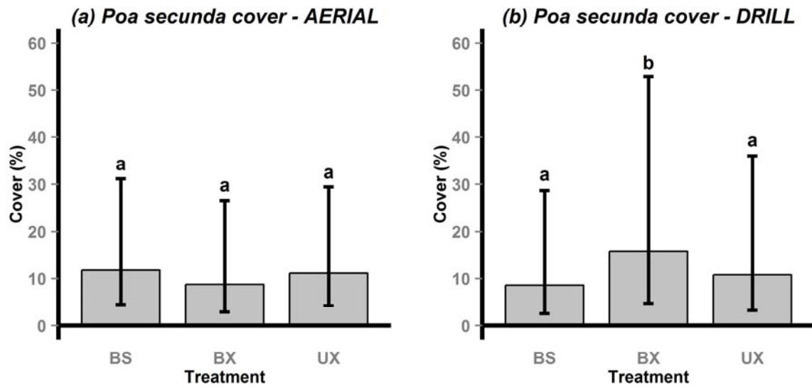
Fig. S5. Cover of Poa secunda at aerial (a) and drill (b) seedings where P. secunda was seeded ( n = 3 and n = 10 for aerial and drill seedings, respectively; Table 2). Different letters represent significant differences ( P < 0.05 ) between treatments. Error bars are 95% confidence intervals.
