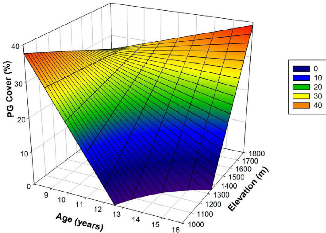
Fig. S3. Model of predicted perennial grass (PG) cover across age and elevation for the burned-seeded (BS) treatment of aerial seedings. An interaction between age and elevation was present. Elevation was truncated at 1000 and 1800 m and age was truncated at 8 and 16 years to stay within a region of higher confidence in the predictions. Heat load, which also affected aerial PG cover (see Table 3), was held constant at an intermediate level (0.94) for modeled predictions. Cover values grade above and below the color and cover values in the legend.
