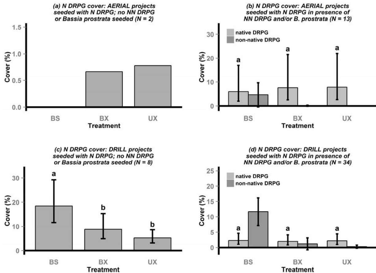
Fig. S4. Cover of native deep-rooted perennial grasses (N DRPG) at aerial (a, b) and drill (c, d) seedings where N DRPG were seeded in the absence (a, c) or presence (b, d) of seeded, introduced species (non-native deep-rooted perennial grasses (NN DRPG) and/or Bassia prostrata ). For (b) and (d), mean NN DRPG cover is also plotted for reference. Different letters represent significant differences ( P < 0.05 ) between treatments in the N DRPG cover mixed model. Error bars are 95% confidence intervals of the mean. Error bars were omitted for (a) since the sample size was very low (N = 2 seedings).
