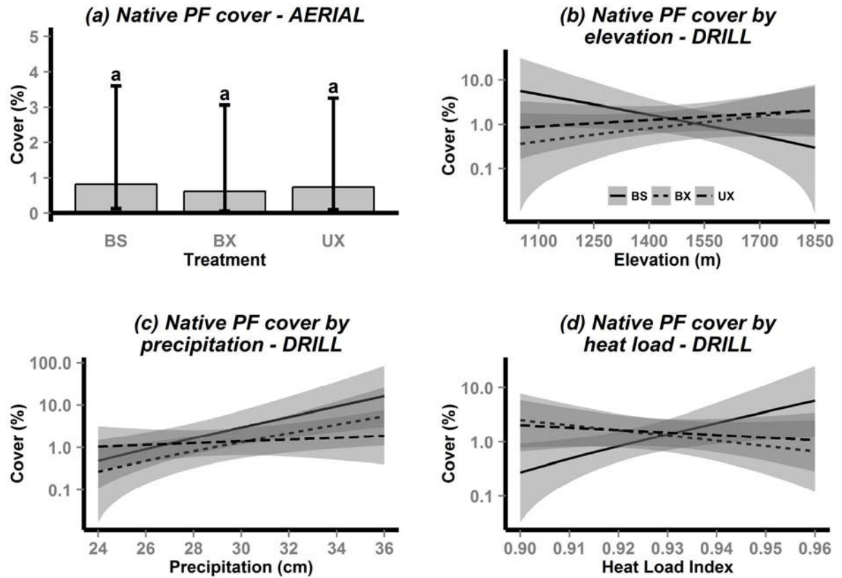
Fig. S6. Cover of native perennial forbs (PF) at aerial (a) and drill (b-d) seedings where the life-form was seeded. Native perennial forb cover at drill seedings were related to precipitation, elevation, and heat load (Table 3), and each covariate is plotted separately in (b-d) while holding other covariates at intermediate values (precipitation: 28 cm, elevation 1400 m, heat load: 0.94). Different letters represent significant differences ( P < 0.05 ) between treatments. Error bars/bands are 95% confidence intervals.
