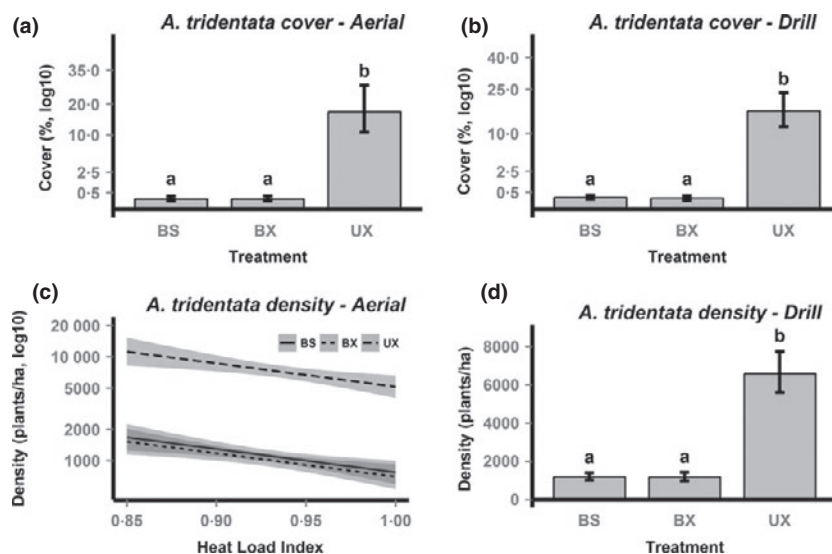
Fig. 4. Artemisia tridentata cover (a, b) and density (c, d) in burned-seeded (BS), burned-unseeded (BX) and unburned (UX) treatments at aerial and drill seeding projects. Different letters represent significant differences ( P < 0.05 ) between treatments. Shaded bands/bars are 95% confidence intervals, and darker areas represent overlap.
