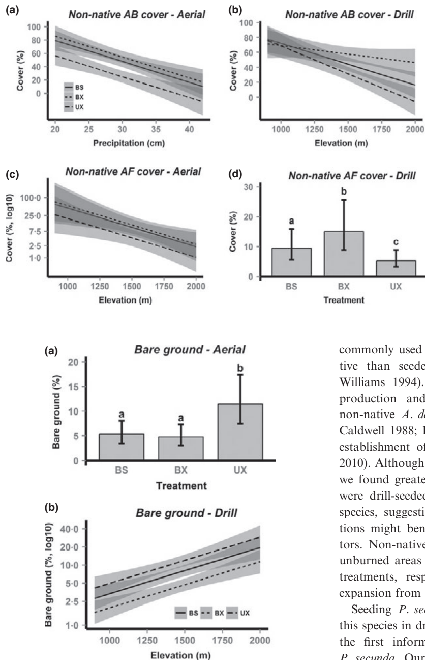
Fig. 7. Percentage bare ground (a, b) in burned-seeded (BS), burned-unseeded (BX) and unburned (UX) treatments at aerial and drill seeding sites. Age of seeding sites also had a significant relationship with percentage bare ground at drill seeding sites (Table 3) and was held constant (12 years since seeding) for predictions in (b). Different letters represent significant differences ( P < 0.05 ) between treatments. Shaded bands/bars are 95% confidence intervals, and darker areas represent overlap.
