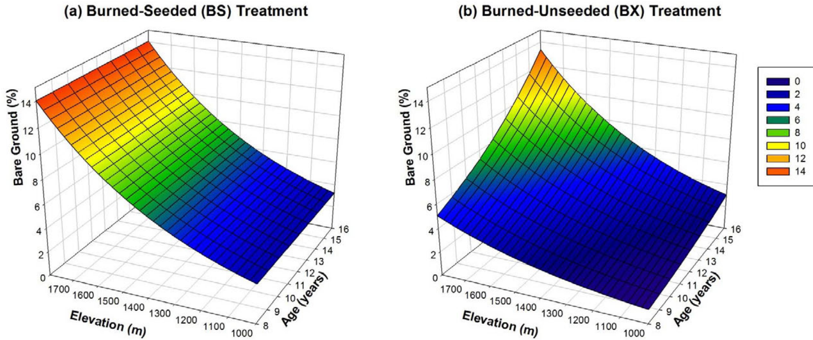
Fig. S7. Model of predicted bare ground (%) in relation to age and elevation at drill seeding burned-seeded (a) and burned-unseeded (b) treatments. An interaction between age and treatment was present in the model (see Table 3). Elevation was truncated at 1000 and 1800 m and age was truncated at 8 and 16 years to stay within a region of higher confidence in the predictions. Cover values grade above and below the color and cover values in the legend.
