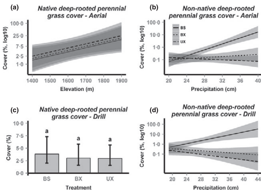
Fig. 3. Native and non-native deep-rooted perennial grass (DRPG) cover in burned-seeded (BS), burned-unseeded (BX) and unburned (UX) treatments at aerial (a, b) and drill (c, d) projects. For drill-seeded non-native DRPG (d), other significant model covariates (Table 3) were held constant at intermediate values (see Fig. 2). Different letters represent significant differences ( P < 0.05 ) between treatments. Shaded bands/bars are 95% confidence intervals, and darker areas represent overlap.
