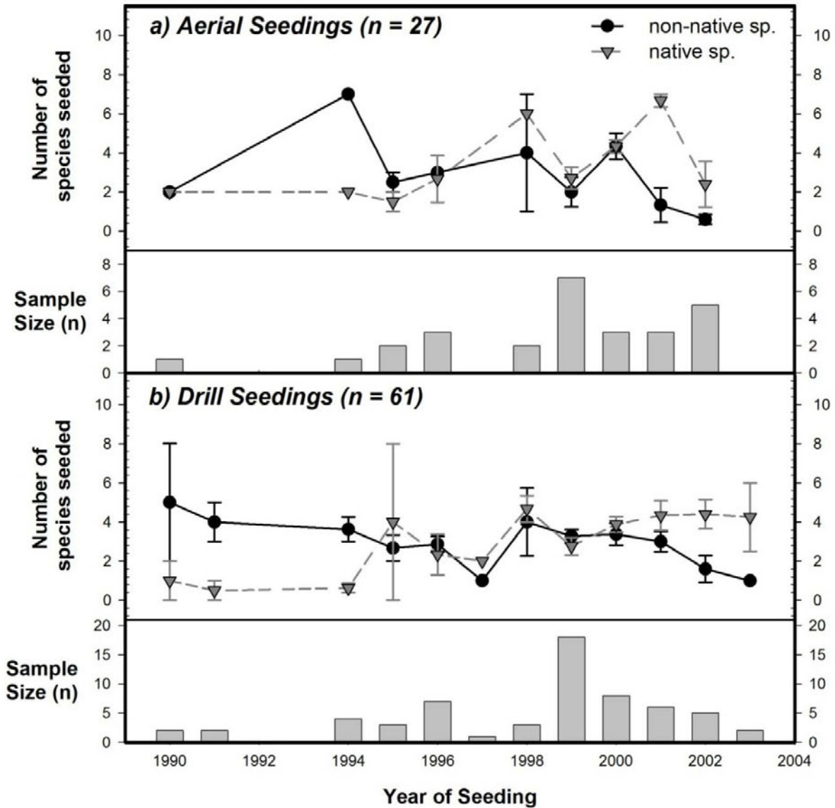
Fig. S1. Trends by year from 1990-2003 in the quantity of sites sampled and the mean number of native or non-native species seeded at aerial (a) and drill (b) seedings. Native and non-native species seeded are according to BLM records of ESR seedings. Error bars are one standard error (SE) of the mean.
