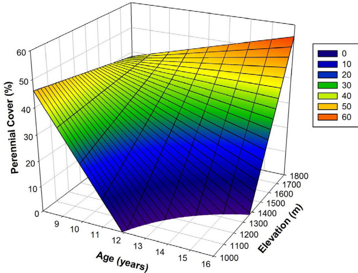
Fig. S2. Model of predicted total perennial plant cover across age and elevation for the burned-seeded (BS) treatment of aerial seedings. An interaction between age and elevation was present (see Table 3). Elevation was truncated at 1000 and 1800 m and age was truncated at 8 and 16 years to stay within a region of higher confidence in the predictions. Cover values grade above and below the color and cover values in the legend.
