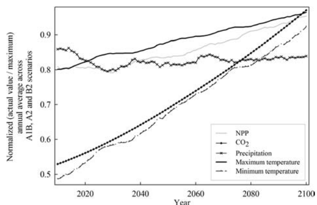
Fig. 3 Normalized 10-year moving average of trends in annualized NPP, \text{CO}_2 , precipitation, maximum temperature, and minimum temperature
