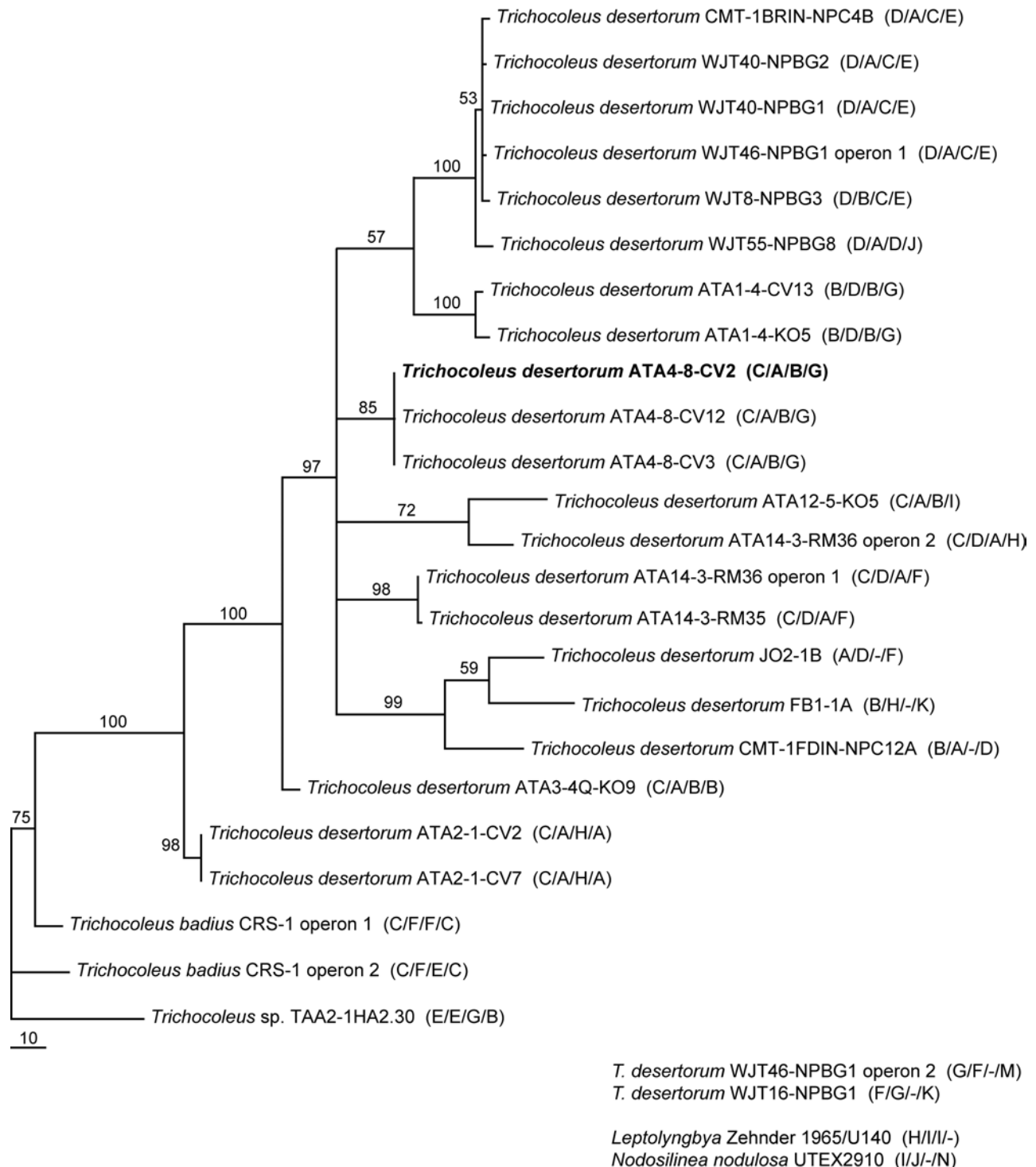
FIGURE 5. Phylogenetic relationships among Trichocoleus strains based on parsimony analysis with 16S–23S ITS region sequence. Values above branches represent bootstrap values from this analysis. Holotype is based on strain in bold font. Letters in parentheses represent ITS helices shown in Figs. 6–9 in order: D1–D1'/Box-B/V2/V3. Helix pattern for operons not included in the ITS tree are shown in lower right corner.
