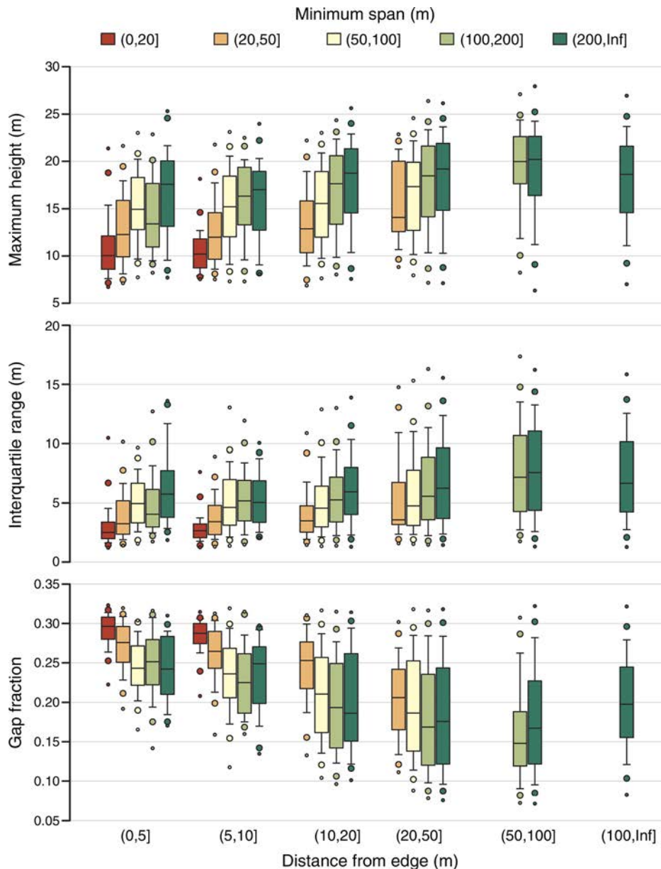
FIG. 6. Boxplots of canopy structure response variable distributions along distance from edge and selected minimum span values from fragments sampled across the study landscape on Mauna Loa volcano, Hawai'i Island. Large dots represent the 5th and 95th percentiles, and small dots represent the 1st and 99th percentiles. The line inside the box is the median. Upper and lower end points are the 75th and 25th percentiles, respectively. Whiskers are the 10th and 90th percentiles. Inf is positive infinity.
