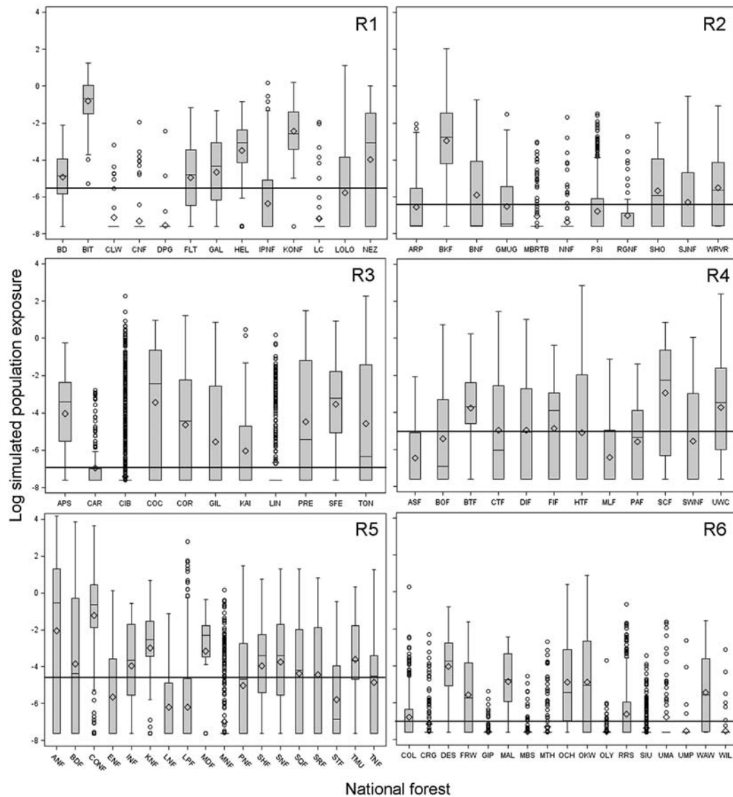
Fig. 10. Box plots of log transformed simulated population exposure on the 82 national forests (NF) in the western US. Simulated population exposure was calculated from population density for WUI multiplied by the proportion of WUI burned by fires ignited on NF. Population data are from LandScan USA (2009) . Fire perimeters were derived from FSIM fire perimeter outputs ( Finney et al., 2011 ). Individual WUIs were assigned to the closest NF.
