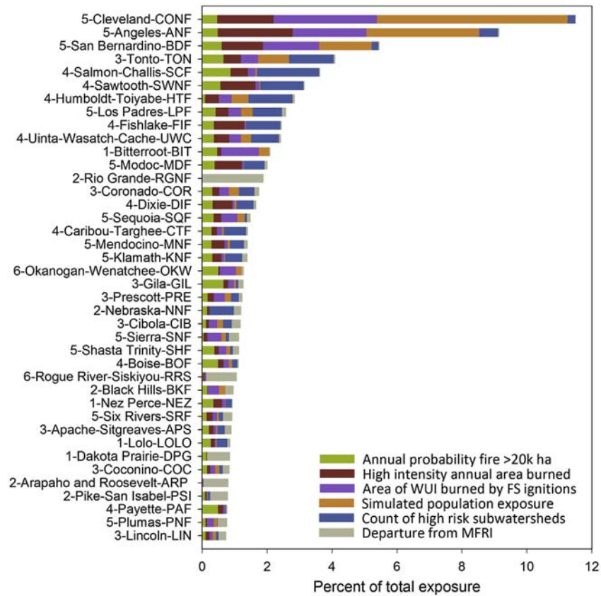
Fig. 11. Ranking results for the top 50% of western national forests (out of the 82 included in the study) in terms of six wildfire exposure variables from simulation outputs. The ranking was performed with simulation outputs since empirical data are insufficient to obtain robust estimates of key exposure parameters. The length of the bar represents the percentage contribution to the total westwide exposure for each metric. Numbers on the y-axis indicate region. See Section 2 for detailed descriptions of wildfire exposure variables included.
