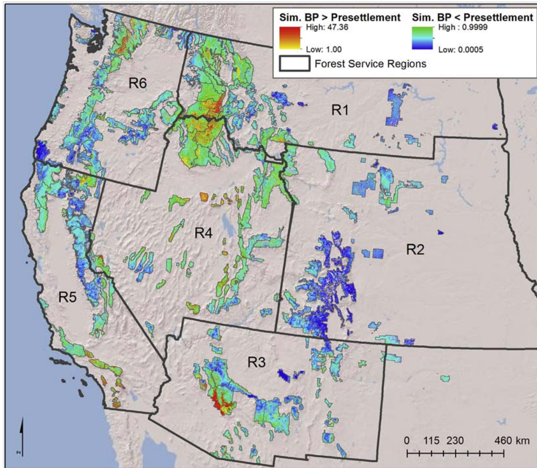
Fig. 5. Map of the ratio of simulated burn probabilities to derived pre-European settlement burn probabilities based on LANDFIRE (2013b) mean fire return interval (MFRI) for the 82 western national forests.
