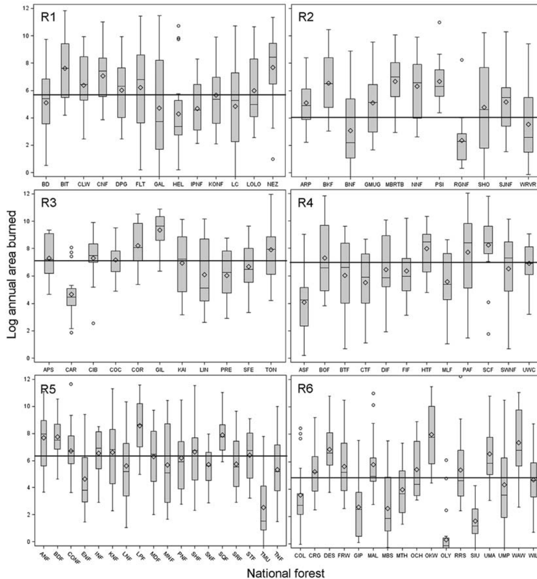
Fig. 2. Box plots of log transformed annual area burned on the 82 national forests in the western US grouped by US Forest Service region. Diamonds indicate Forest means; thick black horizontal line indicates regional average. Data are from Short (2013) for the period 1992–2009. Note that fires that burned onto a Forest from ignitions outside the Forest boundary were not included in the calculations.
