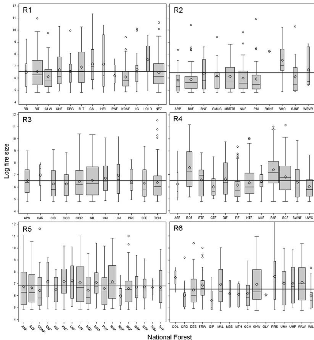
Fig. 3. Variable width box plots of log transformed fire size by national forest for the 82 national forests in the western US grouped by US Forest Service region. Width of the box indicates the relative number of fires. Diamonds indicate Forest means; thick black horizontal line indicates regional average. Data are from Short (2013) for the period 1992–2009. Average fire size excludes fires <121 ha.
