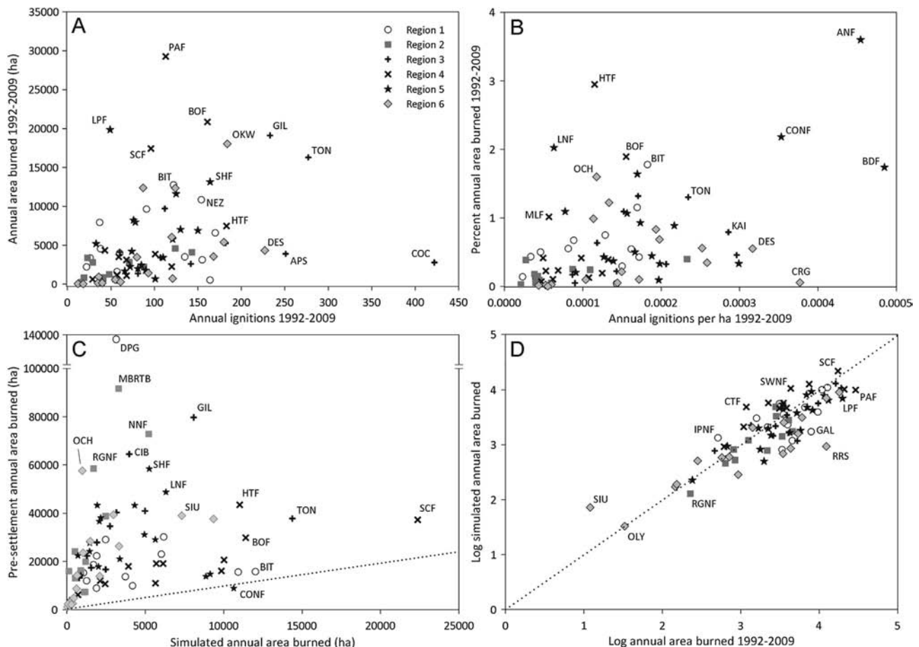
Fig. 4. Comparison of pre-settlement, recent, and simulated fire statistics by national forest (NF). (A) Recent annual area burned versus recent ignitions. Data include area burned off and within NFs from ignitions within NFs. (B) Percent area burned versus annual ignitions per hectare by Forest and region. Area burned off national forests from fires ignited on Forests was removed using land ownership data in the database. Note that area burned by fires that burn onto NF but were ignited outside NF boundaries was not counted. (C) Simulated annual area burned versus pre-European settlement expected annual area burned based on LANDFIRE (2013a) mean fire return interval (MFRI). Note break in y-axis. (D) Log transformed simulated annual area burned versus log transformed recent annual area burned. Simulated data in (C) and (D) include all area burned by fires (NF and non-NF) ignited within NFs. The dotted line in panels C and D represent the 1:1 ratio between the axes.
