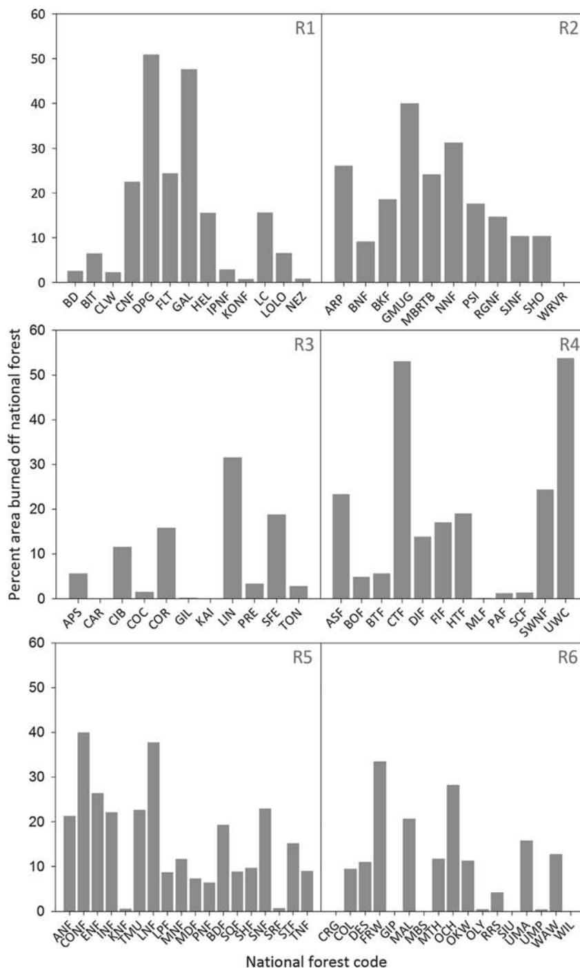
Fig. 8. Percent of non-Forest Service land burned by recent fires that ignited within national forests. Data are from FIRESTAT (2011) and include ignitions from 1990 to 2011 for fires >405 ha.
