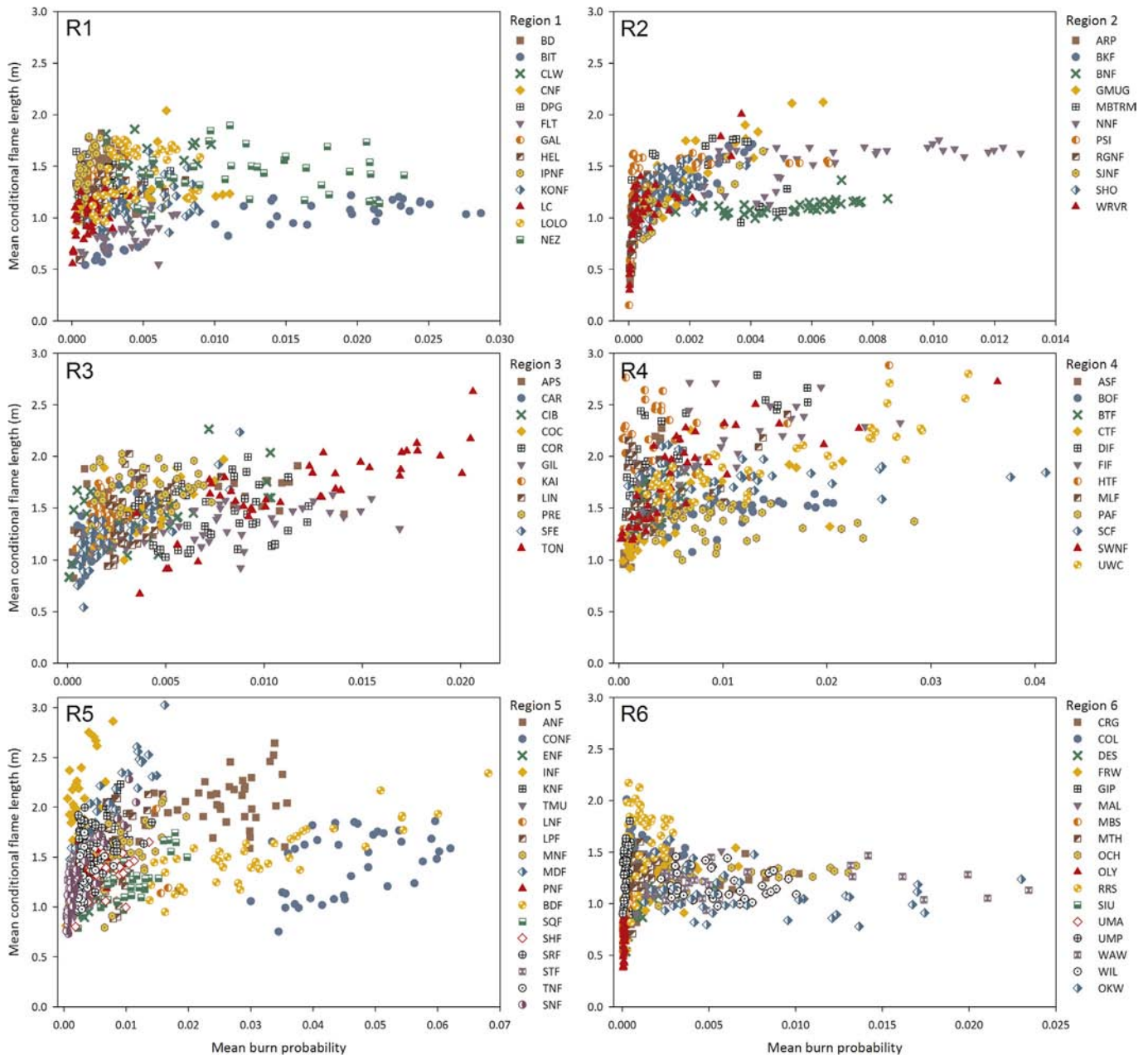
Fig. 7. Scatter plot of average conditional flame length versus burn probability for a random sample of 40 12-digit subwatershed HUCs by Forest and region in the western US. Outputs are derived from the flame length probability files in FSIM (Finney et al., 2011). Burned area estimated for fires that ignited both within and outside national forests. Note: Late Tahoe Basin (TMU) contains only four subwatersheds and Columbia River Gorge (CRG) contains only 17 subwatersheds.
