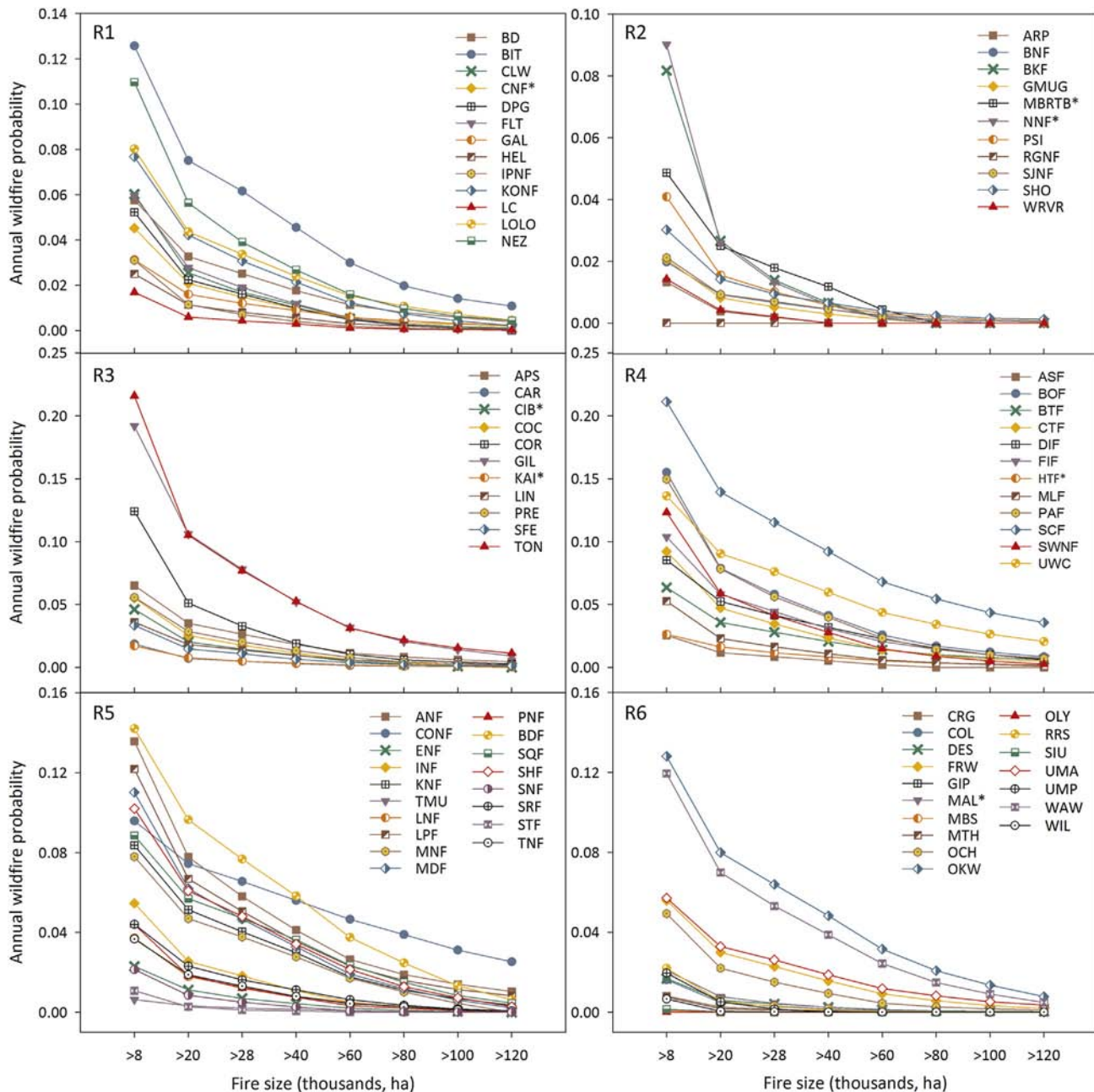
Fig. 6. Simulated annual probability of a wildfire of a given fire size assuming ca. 2008 landscape conditions and contemporary weather patterns by Forest and region in the western US. Data were calculated from the FSIM fire list outputs from Finney et al. (2011) and include area burned off national forests in the simulation. Asterisks indicate Forests that spanned multiple Fire Planning Units. See Section 2.8 for details. Note differing scales on the y-axes.
