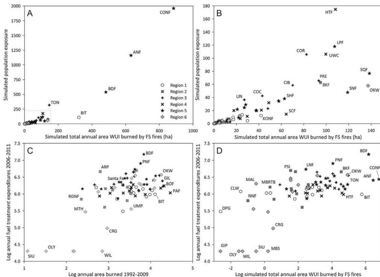
Fig. 9. (A) Average simulated annual area of Wildland Urban Interface (WUI) burned by fires ignited on national forests (NF) derived from FSIM fire perimeter outputs (Finney et al., 2011) versus average simulated population exposure. Simulated population exposure was calculated from population density for WUI multiplied by the proportion of WUI burned by fires ignited on NF. Population data are from LandScan USA (2009). Individual WUIs were assigned to the closest NF. Note break in y-axis. Dotted line box indicates graph area displayed in panel B. (B) Average simulated annual area of WUI burned versus average simulated population exposure, graphed to exclude outliers visible in panel A. (C) Average annual fuel treatment expenditures versus recent area burned. Recent data are from Short (2013) and include ignitions from 1992 to 2009. Data include all area burned by fires that ignited within NF. (D) Average annual fuel treatment expenditures versus average simulated annual area of WUI burned by fires ignited on NF. See Section 2.4 for details on fuel treatment expenditure data.
