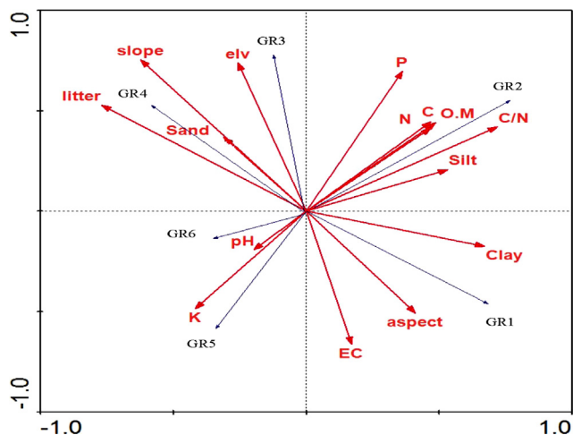
Fig. 4. Ordination diagram showing the result of CCA analysis of vegetation and environment variables in the study area. Abbreviations of vegetation and environment variables: GR = Group, elv = Elevation.
