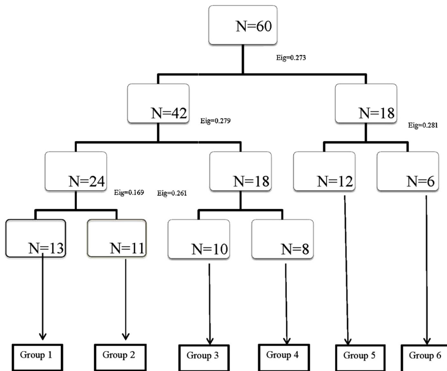
Fig. 3. Diagram of TWINSpan analyses on 60 sample plots in study area.
