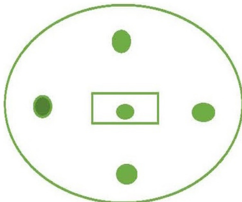
Fig. 2. Fill points are soil sample location and rectangular is herbaceous layer sample location.
