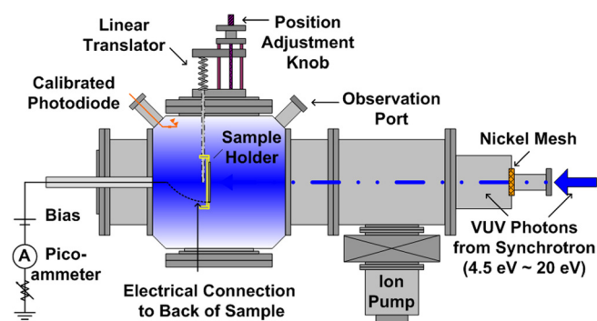
FIG. 2. Schematic of the synchrotron vacuum ultraviolet irradiation system used in this work.
