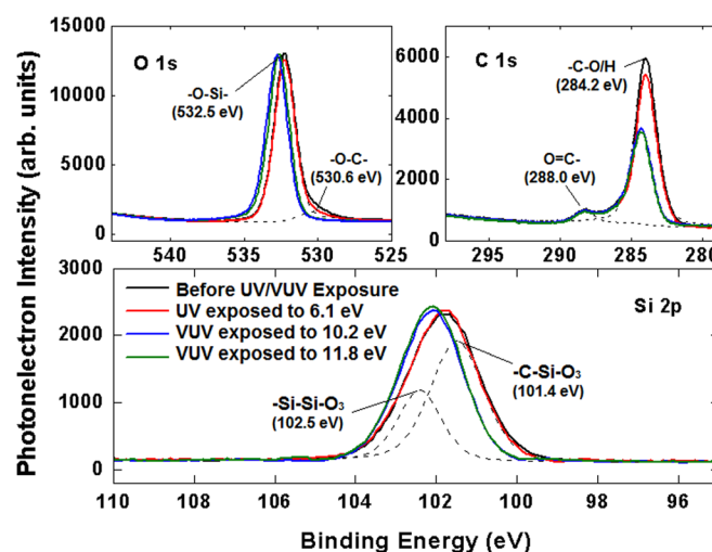
FIG. 8. XPS spectra showing the changes of O 1s, C 1s, and Si 2p electron orbitals of as-deposited samples after synchrotron irradiation several different photon energies. The dashed lines are the deconvolution results after fitting the spectrum with the Gaussian peaks of the unexposed samples.
