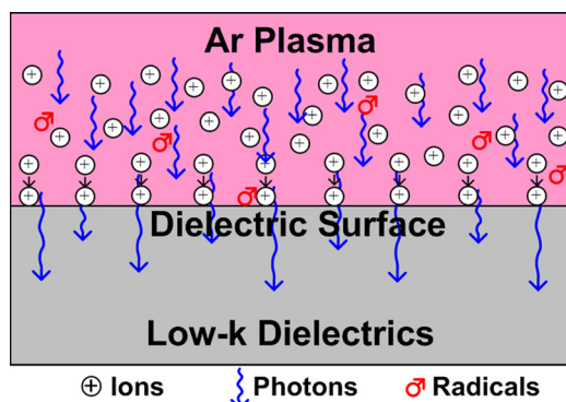
FIG. 3. Schematic drawing of surface/bulk modification effect of argon plasma on the dielectric films.
