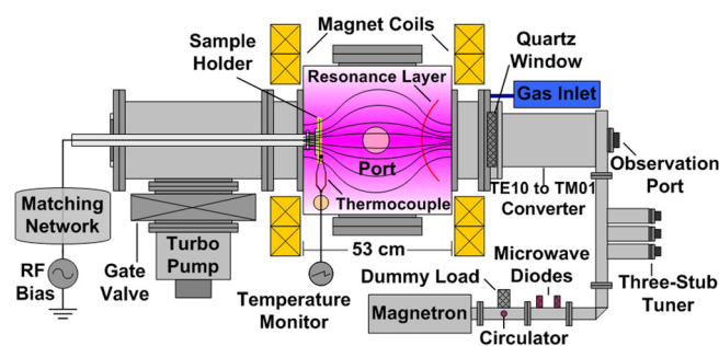
FIG. 1. Schematic of the electron cyclotron resonance plasma reactor apparatus used in this work.
