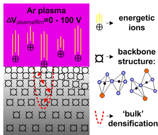
FIG. 6. Model of physical ion bombardment induced film bulk densification.
