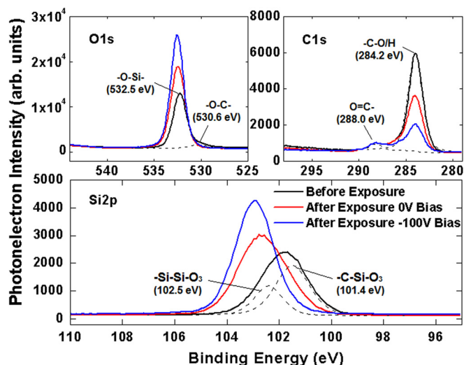
FIG. 5. XPS spectra showing the changes of O 1s, C 1s, and Si 2p electron orbitals of as-deposited samples after plasma exposure with floating potential or a -100 V DC bias applied to the sample chuck. The dashed lines are the deconvolution results after fitting the spectrum with the Gaussian peaks of the unexposed samples.
