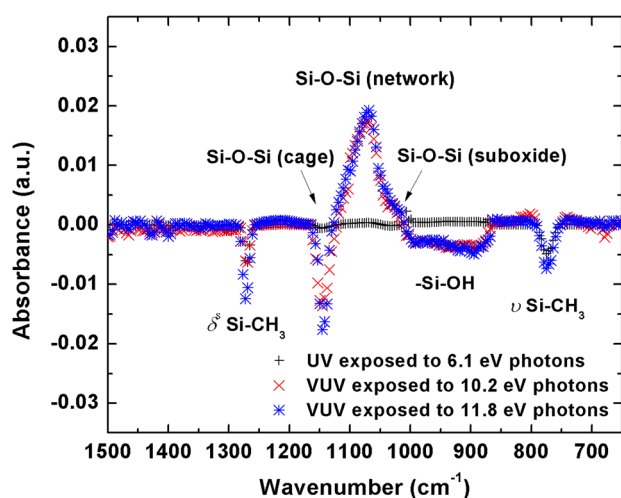
FIG. 7. Differential FTIR spectrum of porous organosilicate dielectric irradiated by synchrotron with several photon energies. Here, “ \delta ” corresponds the bending vibrational mode and “ \nu ” corresponds the stretching vibrational mode.
