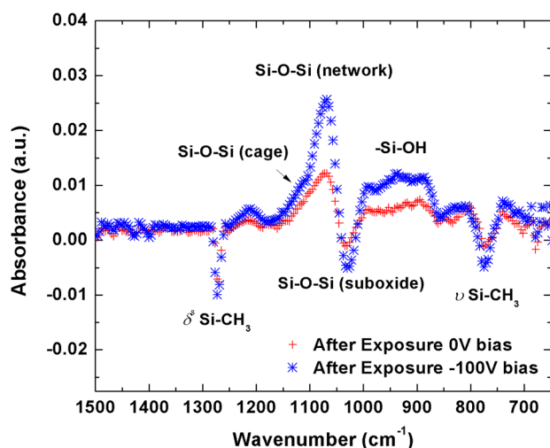
FIG. 4. Differential FTIR spectrum of plasma-exposed porous organosilicate dielectric films with floating potential or a -100\text{ V} DC bias applied to the sample chuck. Here, " \delta^{\text{Si-CH}_3} " corresponds the bending vibrational mode and " \nu " corresponds the stretching vibrational mode.
