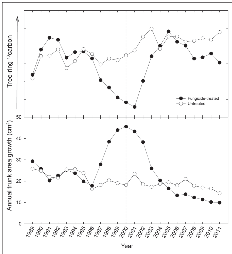
Building on a previous study that applied fungicide (from 1996 to 2000) to infected Douglas-firs, researchers returned to the study site and took core samples to analyze the tree rings for the abundance of the ^{13}\text{C} isotope. This confirmed that when Swiss needle cast symptoms were minimized, ^{13}\text{C} was less abundant in the tree rings and annual trunk growth increased.
