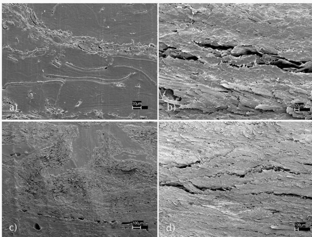
Fig. 4. Micrographs of dry panels (a and c) water soaked panels (b and d)
