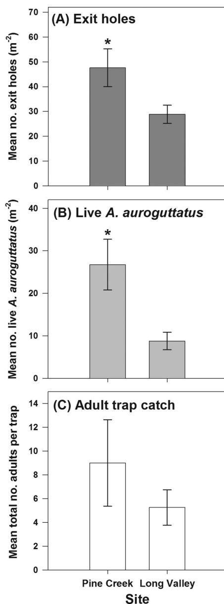
Fig. 3. Mean density of A. auroguttatus (A) exit holes on Q. agrifolia for all months, (B) within-tree immatures during months when adults were not flying (i.e., all months except May–October), and (C) mean total number of adult A. auroguttatus caught per trap from four traps at each site May–October, 2011. *Indicates statistical significance according to Welch's t -tests. Sample sizes are: Pine Creek = (A) 45 and (B) 25 trees; Long Valley = (A) 52 and (B) 33 trees.
