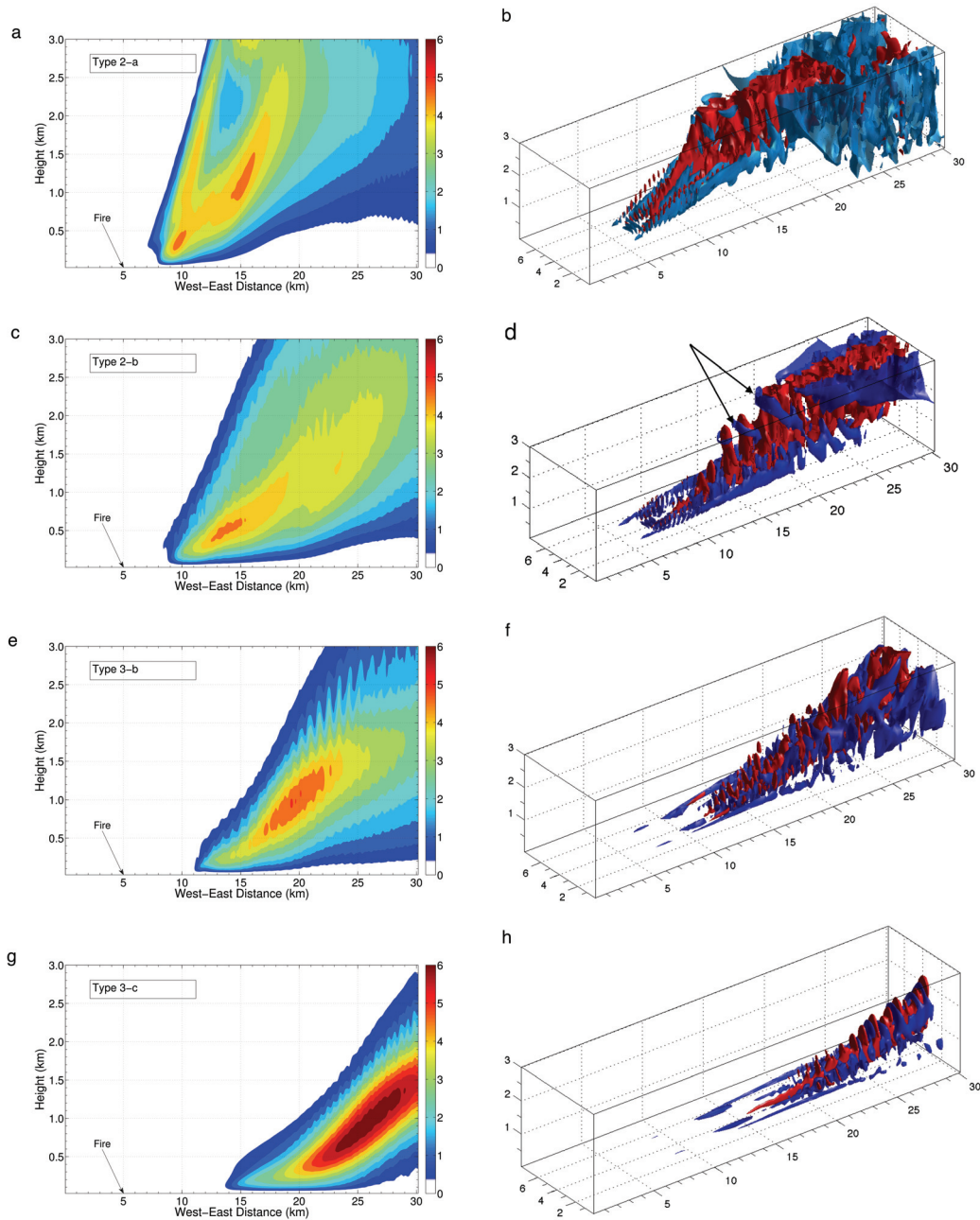
Figure 3. Left column: time-averaged (from 1 min model output over 2 hr) w -velocity from a x - z cross section along the fire's central line running west to east of the domain. Right column: a snapshot iso-surface (at 2 hr) of the w -velocity at 3 \text{ m s}^{-1} (red) and -1.5 \text{ m s}^{-1} (blue).
