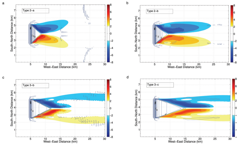
Figure 2. Time-averaged (from 1 min model output over 2 hr) v -velocity component (south-north) colour-shaded contours overlaid with contour lines (2 K interval) of potential temperature for an x - y cross section at 10 m AGL.
