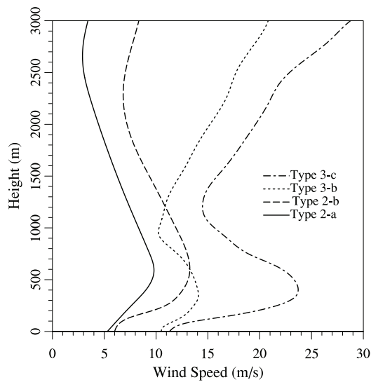
Figure 1. Background wind speed profiles used in the four numerical simulations, up to a height of 3000 m AGL. They correspond to the type 2-a, 2-b, 3-b and 3-c Byram (1954) wind profiles.
