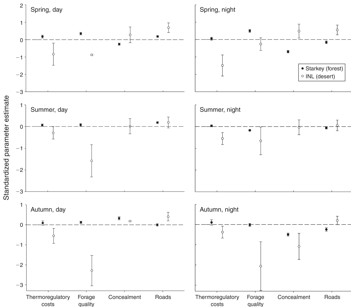
FIG. 2. Model-averaged, standardized parameter estimates (with 95% confidence intervals) obtained from resource selection functions for North American elk ( Cervus elaphus ) during daytime and nighttime hours in spring (April–June), summer (July–September), and autumn (October–November), 2010–2012, at the Starkey Experimental Forest and Range, Oregon, USA ( n = 86 elk), and the Idaho National Laboratory Site, Idaho, USA ( n = 35 elk). Predictor variables included energy and water costs imposed by the thermal environment (Thermoregulatory costs), forage quality, concealment cover (Concealment), and distance to roads (Roads). Resource selection functions were derived from generalized linear mixed models fit to used and random locations from each study site. Concealment cover was not included in the summer model for Starkey, because it was correlated with forage quality ( r > 0.6 ).
