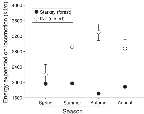
FIG. 3. Daily energy expended on locomotion (mean and 95% CI) by North American elk ( Cervus elaphus ) during spring (April–June), summer (July–September), and autumn (October–November), 2010–2012, at the Starkey Experimental Forest and Range, Oregon, USA ( n = 86 elk; mean body mass = 219.9 kg), and the Idaho National Laboratory Site, Idaho, USA ( n = 35 elk; mean body mass = 241.6 kg). Mean values across all three seasons also are presented (annual).
