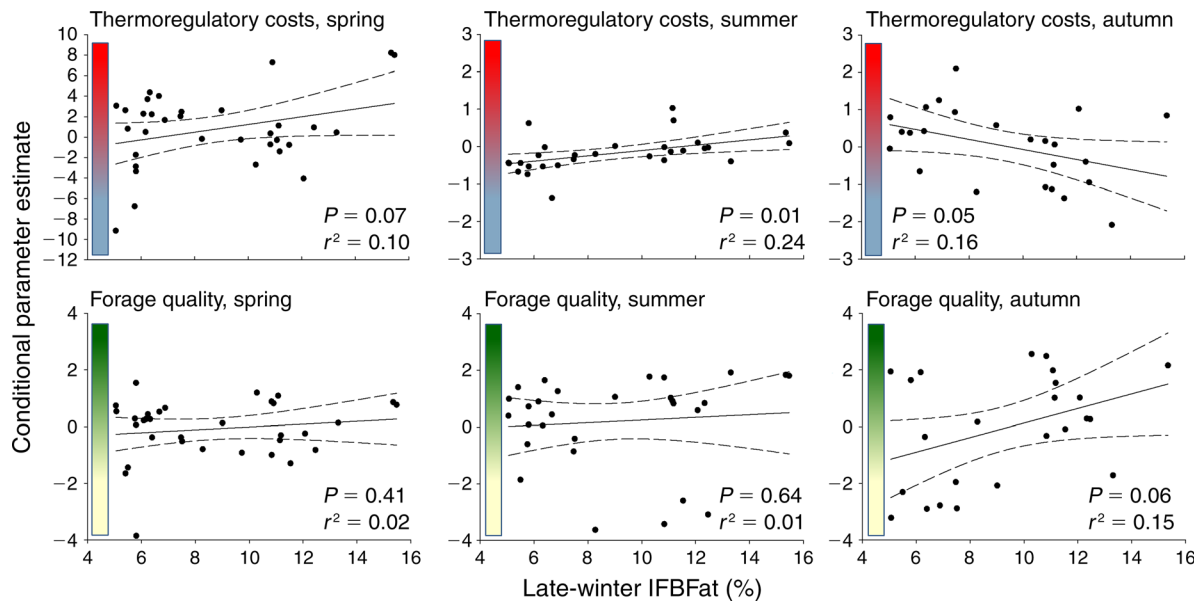
FIG. 5. Conditional (individual-level) parameter estimates from resource selection functions for North American elk during spring (April–June), summer (July–September), and autumn (October–November), 2010–2012, in the desert site (Idaho National Laboratory). Parameter estimates are plotted against late-winter nutritional condition (percentage ingesta-free body fat in February or March; IFBFat) and indicate, for each individual, the relative strength of selection for areas that reduced costs of thermoregulation (selection for lower cost, blue; selection for higher cost, red), or increased access to high-quality forage (selection for lower quality, yellow; selection for higher quality, green). Resource selection functions were derived from generalized linear mixed models fit to used and random locations from each study site. Fitted lines from simple linear regression analyses are shown, along with 95% confidence intervals (dashed lines) and test results.
