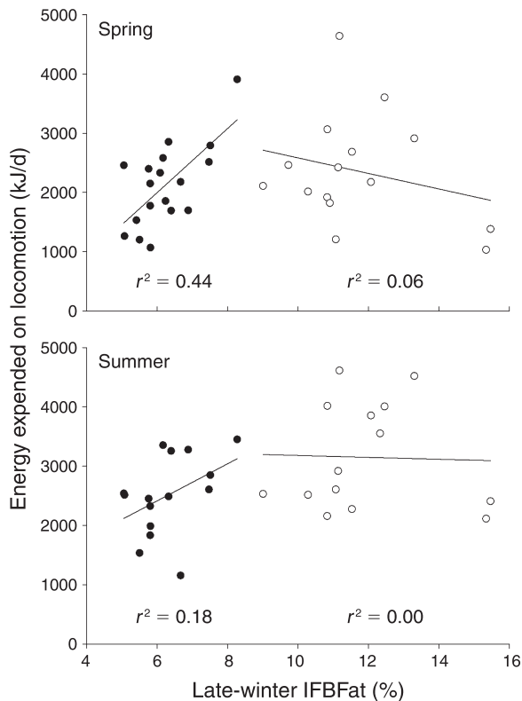
FIG. 6. Piecewise linear regressions of mean daily energy expended on locomotion by North American elk (mean body mass = 241.6 kg) against late-winter nutritional condition (percentage ingesta-free body fat in February or March; IFBFat) during spring (April–June) and summer (July–September), 2010–2012, in the desert site (Idaho National Laboratory). Breakpoints (at ~8% ingesta-free body fat in both seasons) and slopes were estimated iteratively (Bates and Watts 1988, Ryan and Porth 2007). Below the breakpoint (solid circles), energy expended on locomotion was positively related to nutritional condition (i.e., individuals in better condition expended more energy on locomotion), whereas above that level (open circles), energy expended on locomotion was unrelated to condition.
