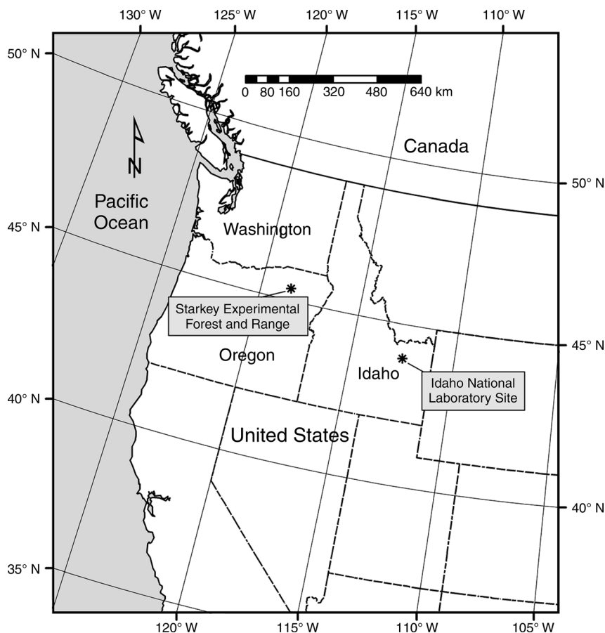
FIG. 1. The locations of our study areas: the Starkey Experimental Forest and Range in northeastern Oregon (temperate, montane forest), and the Idaho National Laboratory Site (an arid, high-elevation desert) in southeastern Idaho, USA.
