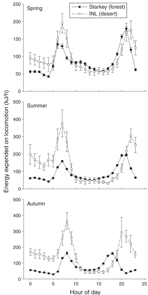
FIG. 4. Energy expended on locomotion (mean and 95% CI) by North American elk on an hourly basis throughout the day during spring (April–June), summer (July–September), and autumn (October–November), 2010–2012, at the Starkey Experimental Forest and Range, Oregon, USA ( n = 86 elk), and the Idaho National Laboratory Site, Idaho, USA ( n = 35 elk). Hour 0 begins at 12:01 hours.
