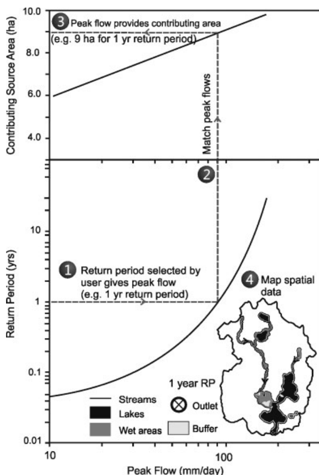
Figure 4. Principles 4 and 5: Respect temporal variability and spatial heterogeneity of hydrological systems. This hypothetical nomogram illustrates how management plans can be based on the return period of peak flows (temporal variation) and their associated contributing source areas (spatial variation). Cut block, road, or buffers could then be designed based on the degree of risk (i.e., return period of soil saturation or inundation) that the manager is prepared to accept (modified from Krezek, 2001, and Creed et al. , 2008)
