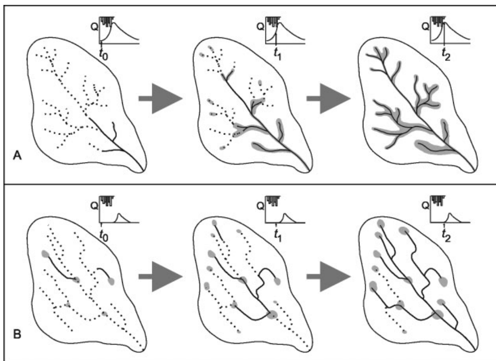
Figure 3. Principle 3: Maintain hydrological connectivity among the critical hydrological features. Hydrological system (A) exhibits a rapid increase in surface connectivity in response to an event, whereas system (B) exhibits a much lesser degree of surface connectivity with much smaller expansion of its variable source areas. Solid and dotted lines represent saturated and dry stream channels, respectively. Shaded areas represent surface saturation. The inset hypothetical hydrographs are measured at the basin outlet (from Todd et al. , 2006)
