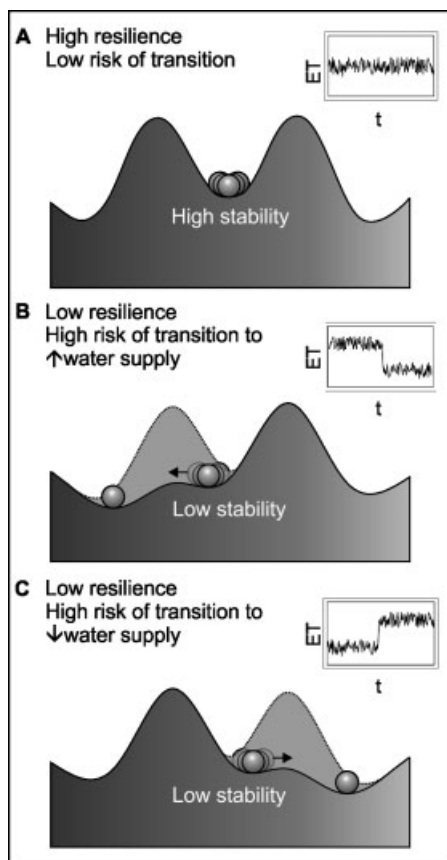
Figure 5. Principle 6: Maintain redundancy and diversity of hydrological form and function. Forest ecosystem stability is defined by the depth of the basin of attraction. A deep basin of attraction (A) indicates a stable ecosystem and one that is resilient to small perturbations. A shallow basin of attraction (B and C) indicates an unstable ecosystem susceptible to a change in state from small perturbations. Forest management practices may reduce the ecosystem's stability (reflected in the shallow basin of attraction) during which small perturbations (arrows) may then force the ecosystem into a change of state. In this example, the ecosystem state is characterized by evapotranspiration (ET); thus, a change in ecosystem state can result in either an increase (B) or a decrease (C) in water production (Q). In (B), changes that reduce ecosystem stability and result in a shift to a decrease in ET (and increase in Q) may include conversion from forest to residential lands (modified from Scheffer, 2010). In (C), changes in forest structure that reduce ecosystem stability and result in a shift to an increase in ET (and decrease in Q) may include forest fire suppression or forest biofuel plantations
