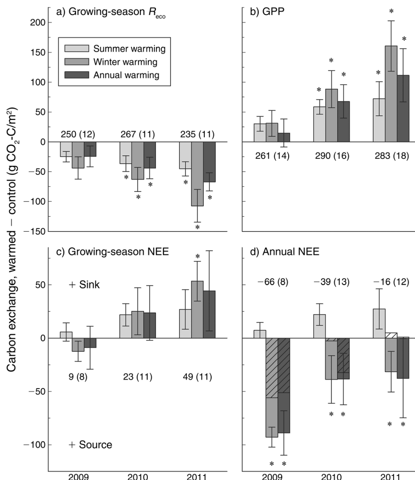
FIG. 1. Effects of soil warming and permafrost thaw (winter warming) and growing-season air warming (summer warming) on cumulative \text{CO}_2 exchange between a tundra ecosystem and the atmosphere. (a) Ecosystem respiration ( R_{\text{eco}} ), (b) gross primary productivity (GPP), (c) growing-season net ecosystem exchange (NEE), and (d) annual NEE were monitored for three years of experimental warming. Annual NEE estimates for winter and annual warming treatments include warming effects from field (January–September) and modeling (October–December) experiments. The hatched bars in panel (d) show annual NEE without autumn–early winter warming (i.e., experimental results only). Bars represent treatment effects on ecosystem \text{CO}_2 exchange: bars above the zero line represent increased ecosystem \text{CO}_2 uptake with warming (“+ Sink” in panel (c)) and below represent increased \text{CO}_2 loss to the atmosphere (“+ Source” in panel (c)). Numbers above/below the zero line are ambient \text{CO}_2 flux values (means with SE in parentheses; \text{g CO}_2\text{-C/m}^2 ). Annual warming represents combined summer and winter warming. An asterisk denotes treatment differences from ambient (paired comparisons, P < 0.05 ).
