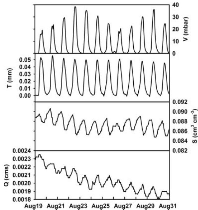
Figure 3. Temporal variation in water fluxes through a small, forested watershed for the period 19–31 August 2000 at the hourly scale. (a) Hourly average vapour pressure deficit ( V , mbar) measured at the nearby primary climate station; (b) hourly total transpiration ( T , mm); (c) hourly soil moisture ( S , \text{m}^3 \text{m}^{-3} ); and (d) hourly total streamflow ( Q , cm)
