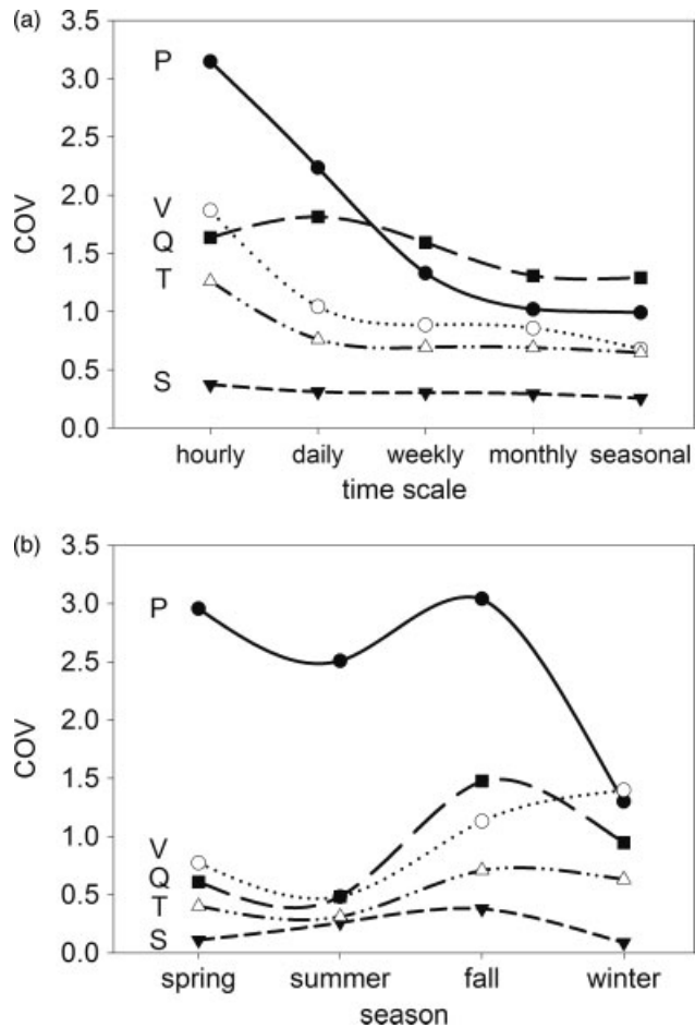
Figure 4. (a) Coefficient of variation by time interval for precipitation (closed circles, solid lines), vapour pressure deficit (open circles, dotted lines), soil moisture (closed inverted triangles, dashed lines), transpiration (open triangles, dash/dot lines), and streamflow (closed squares, long dashed lines) at hourly, daily, weekly, monthly, and seasonal timescales between 1 August 2000 and 30 September 2002 (hourly transpiration only between June and November 2000). (b) Coefficient of variation by season for variables at the daily timescale during the spring (April–May), summer (June–August), fall (September–November), and winter (December–February) based on daily mean values between 13 April 2001 and 1 June 2002
