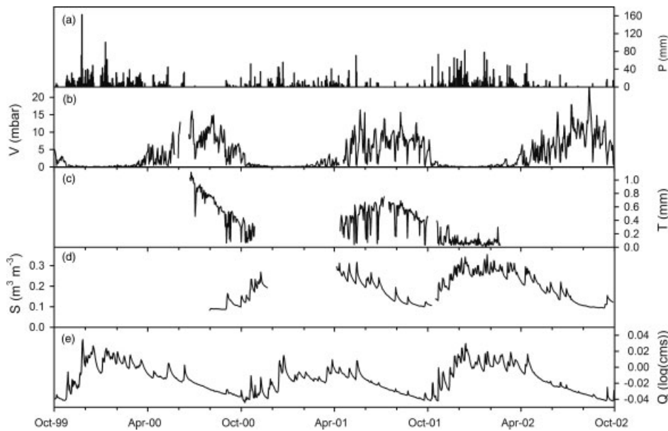
Figure 1. Temporal variation in water fluxes through a small, forested watershed for water years 2000, 2001, and 2002 at the daily scale. (a) Daily total precipitation ( P , mm); (b) daily average vapour pressure deficit ( V , mbar) measured at the nearby primary climate station; (c) daily total transpiration ( T , mm); (d) daily average soil moisture ( S , \text{m}^3 \text{m}^{-3} ); and (e) log-transformed daily average streamflow ( Q , \log(\text{cm}) )
