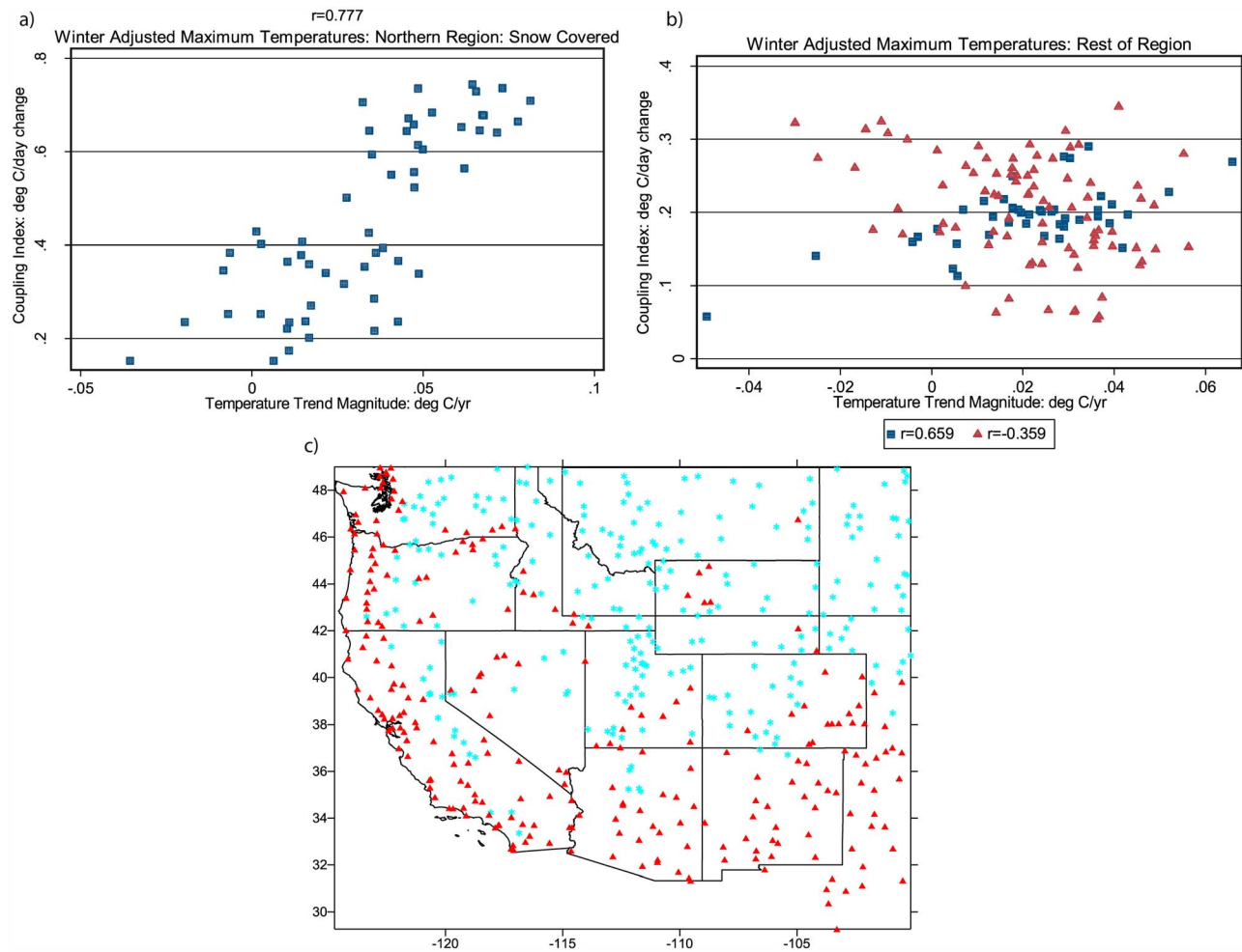
Figure 10. Winter (DJF) adjusted maximum temperature trends versus coupling index for (a) northern tier region east of 115^{\circ}\text{W} and north of 42.5^{\circ}\text{N} only (snow covered) and (b) all other stations including snowy (squares) and nonsnowy (triangles). (c) The location of snowy (snowflake symbol) and nonsnowy (upward triangle) stations in the western United States. A critical threshold of 20 mm was used to separate snowy and nonsnowy locations. The highly coupled northeastern region (used in Figure 10a) is delimited by the box covering parts of Idaho, Montana and Wyoming.
