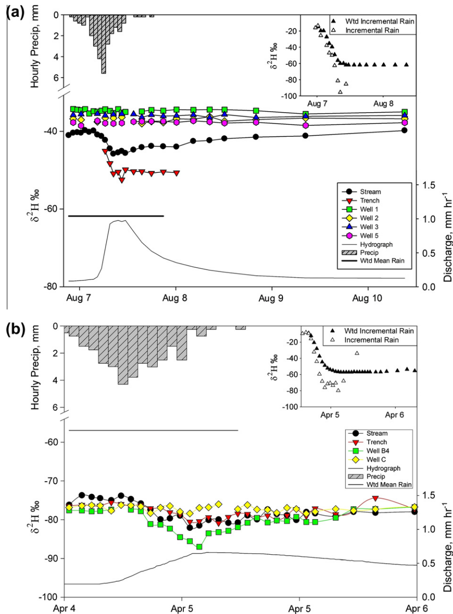
Fig. 6. Stable isotope time series data for sampled storm event at M8 (a) and WS10 (b) with hydrograph and hyetograph. Total storm precipitation was 36 mm at M8 and 34 mm at WS10. The horizontal black line represents total storm weighted mean rain deuterium value. The inset diagrams of each plot display the isotopic values of the high frequency sequential samples of rain water (with each dot representing a point sample taken at hourly increments) in the solid triangles and the calculated incremental mean of the time series during the storm progression shown in the open triangles. Isotope values for some wells at WS10 (b) were not displayed for visual clarity. Those wells are discussed in the text. Wells that accessed deeper bedrock groundwater followed similar trends as Well C, while shallow bedrock wells followed the trend of Well B4.
