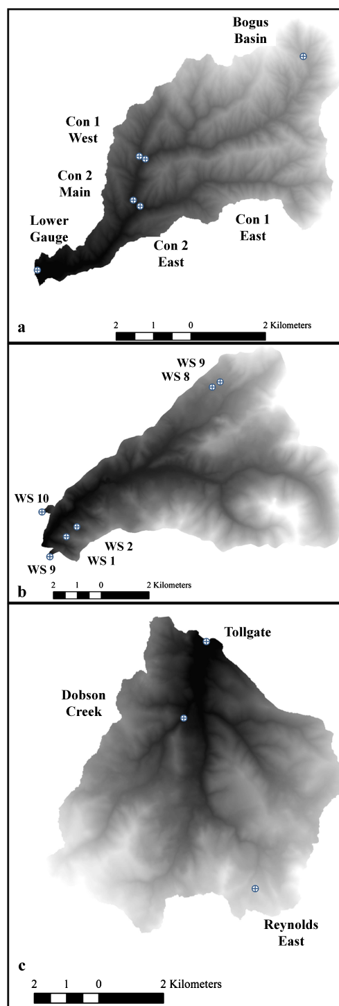
Figure 2. Study locations: (a) Dry Creek, (b) HJ Andrews and (c) Reynolds Creek. Circles indicate locations of gauging stations
