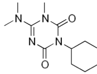
HEXAZINONE
