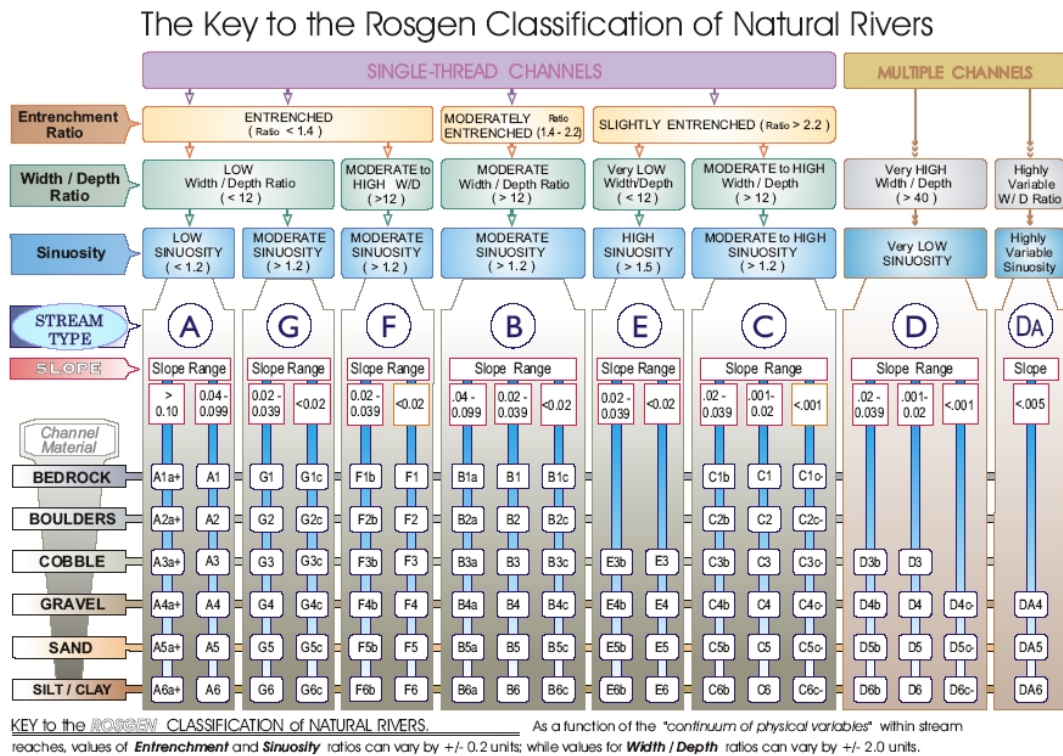
Figure 19. Classification system for natural rivers according to Rosgen (1996) (From Endrenny 2003).
