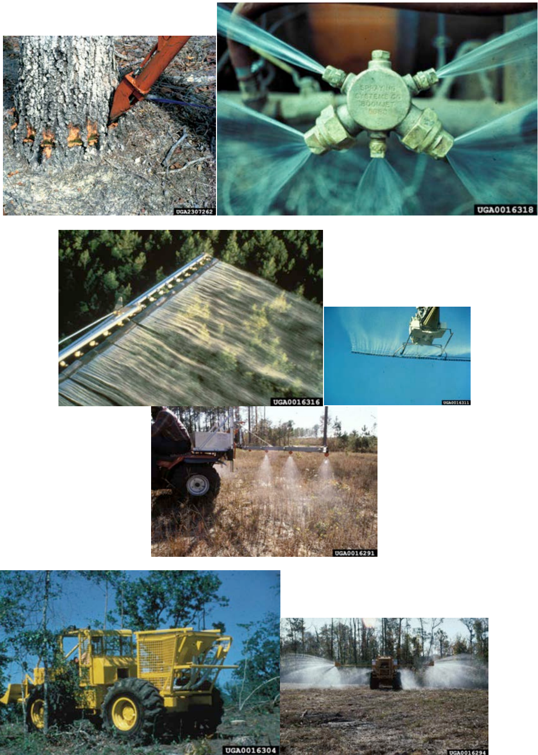
Figure 22. Forestry herbicide application equipment (Photos By James H. Miller, USDA Forest Service, Bugwood.org).
