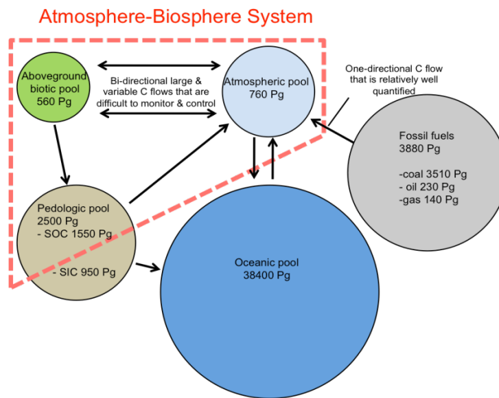
Figure 0.3: The five principal carbon pools and fluxes between them (SOC = soil organic carbon, SIC = soil inorganic carbon). The biosphere and the atmosphere together make up the atmosphere-biosphere system, which is characterised by large bi-directional flows that are highly variable from year to year, difficult to quantify, and expected to be influenced by climate change in ways not yet well understood. In contrast, the flow of carbon from the fossil pool to the atmosphere that is caused by the use of fossil fuels is uni-directional on relevant time scales and better quantified. Atmospheric carbon can - at least temporarily - be re-allocated to the biosphere, but this does not solve the problem of climate change, which is caused mostly by the transfer of fossil carbon into the atmosphere-biosphere system (Berndes et al. , 2011).
