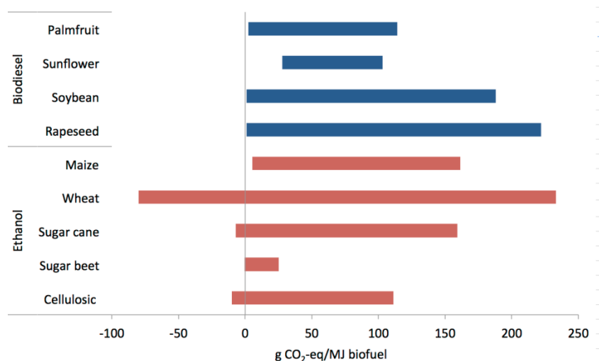
Figure 0.6: Ranges of model-based quantifications of LUC (dLUC + iLUC) emissions associated with the expansion of selected biofuel/crop combinations amortised over 20 years. Based on literature review of LUC modelling in Ahlgren and Di Lucia (2014). Note that there is no statistical processing of data involved, this only shows the range of the reported results in literature, including extreme values. Cellulosic ethanol refers to modelling of switchgrass, miscanthus and maize stover.
