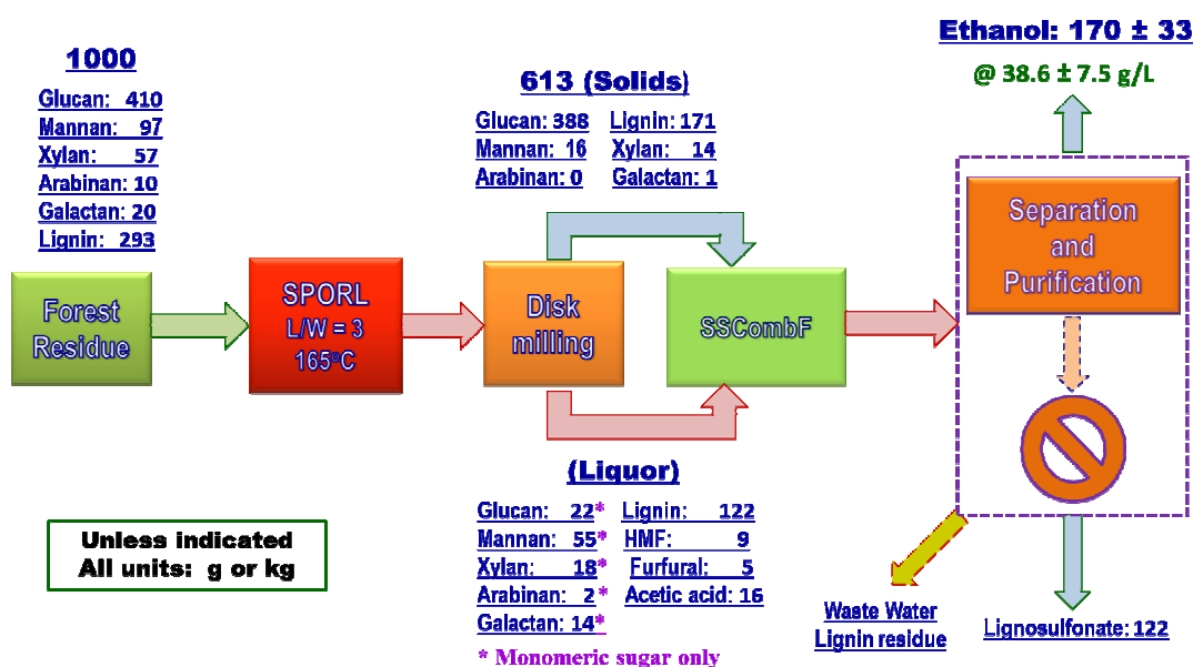
Figure 5: Overall mass balance of the present study
