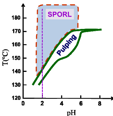
Figure 1: Comparisons of SPORL with sulfite pulping operating conditions
