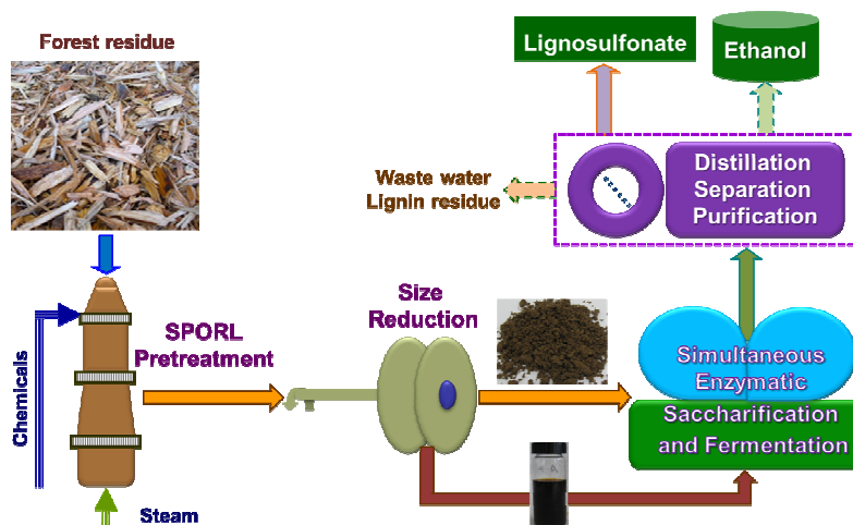
Figure 2: Schematic flow diagram of the experiments
