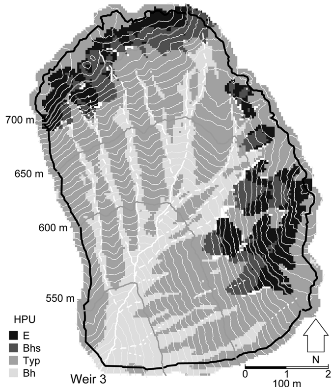
Fig. 9. Map of hydropedologic units (HPUs) of Watershed 3 derived from classifying each cell by the unit most likely to occur in the multinomial logistic regression. Cells where no one HPU was predicted to have an occurrence of 40% or more remained unclassified and are shown as white cells. This map highlights differences in soil formation due to hydropedologic processes, including zones where lateral eluviation (E podzols) or lateral illuviation (Bh's and Bh podzols) vs. vertical podzolization (typical podzols) predominate.
