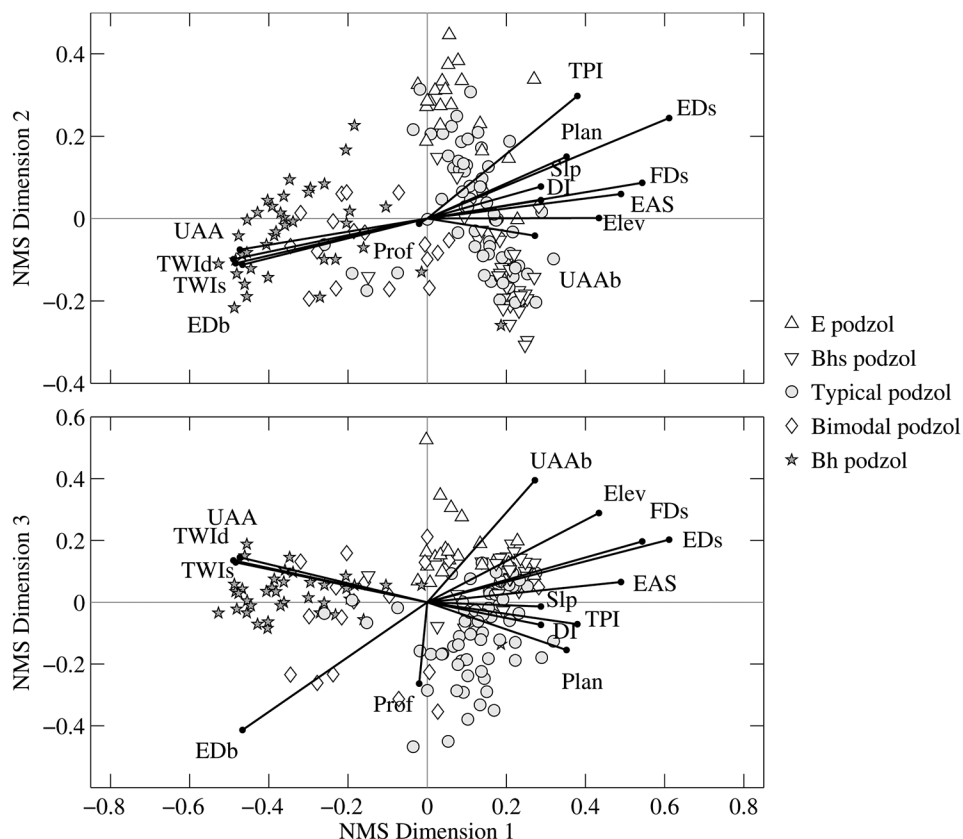
Fig. 4. Nonmetric multidimensional scaling (NMS) ordination using the Bray–Curtis dissimilarity with topographic metrics overlain as Spearman correlates demonstrated hypopedologic unit similarity through clustering in NMS space. Topographic metrics are downslope index (DI), elevation above stream (EAS), Euclidean distance from bedrock outcropping (EDb), Euclidean distance from stream (EDs), elevation (Elev), flow distance from stream (FDs), planform curvature (Plan), profile curvature (Prof), slope (SLP), topographic position index (TPI), topographic wetness index using DI (TWId), topographic wetness index using SLP (TWIs), upslope accumulated area (UAA), and bedrock-weighted upslope accumulated area (UAAb). Bimodal podzols did not cluster in Dimensions 1 and 3, which produced the lowest Kruskal's stress criterion, and were therefore excluded from multinomial logistic regression model development.
