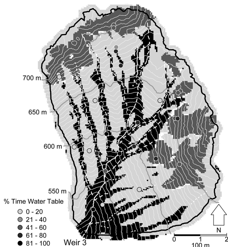
Fig. 10. Map of frequency of water table presence within the solum predicted by logistic regression analysis. White cells indicate areas where no one hydopedologic unit was predicted to have an occurrence of 40% or more and were unclassified. Circles represent measurements of the proportion of the time that the water table was detected above the B–C interface in wells monitored at 10-min intervals for a minimum of 3 yr (Gannon et al., 2104).
