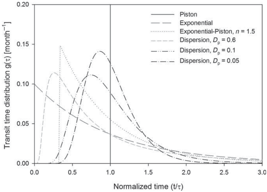
Figure 1. Examples of common MTT distribution functions (TTD) used in FLOWPC simulations.
