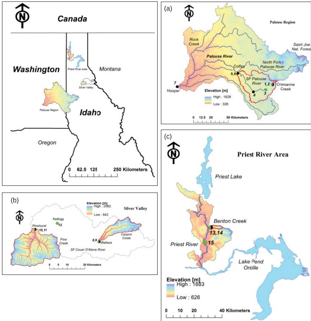
Figure 2. Study watersheds showing elevation (m), main locations and streams, and surface water (black circles) and precipitation (green circles) sampling stations. Semi-filled circles denote stations where both stream and precipitation samples were collected. The inset shows an overview of study area within the inland PNW, USA. (a) PRB includes sampling points 1–2 (Crumaine Creek), 3 (Moscow, ID), 4 (South Fork Palouse River, Pullman, WA), 5–6 (North and South tributaries of the Palouse River), and 7 (Hooper, WA). (b) Pine Creek and Canyon Creek catchments comprise locations 8–9 (Wallace, ID), 10–11 (Pinehurst, ID), and 12 (Kellogg, ID). (c) Lower Priest River watershed includes sampling points 12–14 (Benton Creek), and 5 (Priest River, ID).
