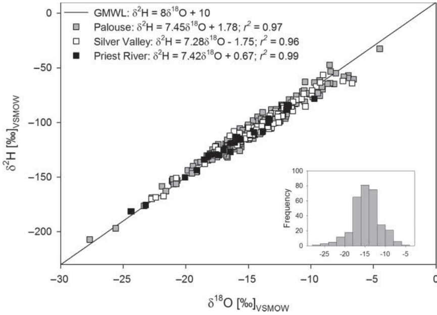
Figure 3. Isotopic composition of precipitation in the inland PNW, USA. Grey squares represent the PMWL ( n = 203 ). Open squares correspond to the SVMWL ( n = 87 ). Black squares denote the Priest River meteoric water line ( n = 26 ). Local meteoric water lines are compared to the GMWL. Inset shows a distribution of \delta^{18}\text{O} values among all the sampling sites.
