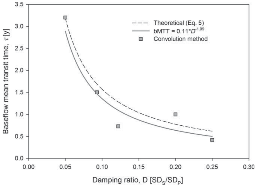
Figure 7. The relationship between baseflow MTT ( \tau ) and the damping ratio of the standard deviations of \delta^{18}\text{O} of stream water ( \text{SD}_s ) to precipitation ( \text{SD}_p ).
