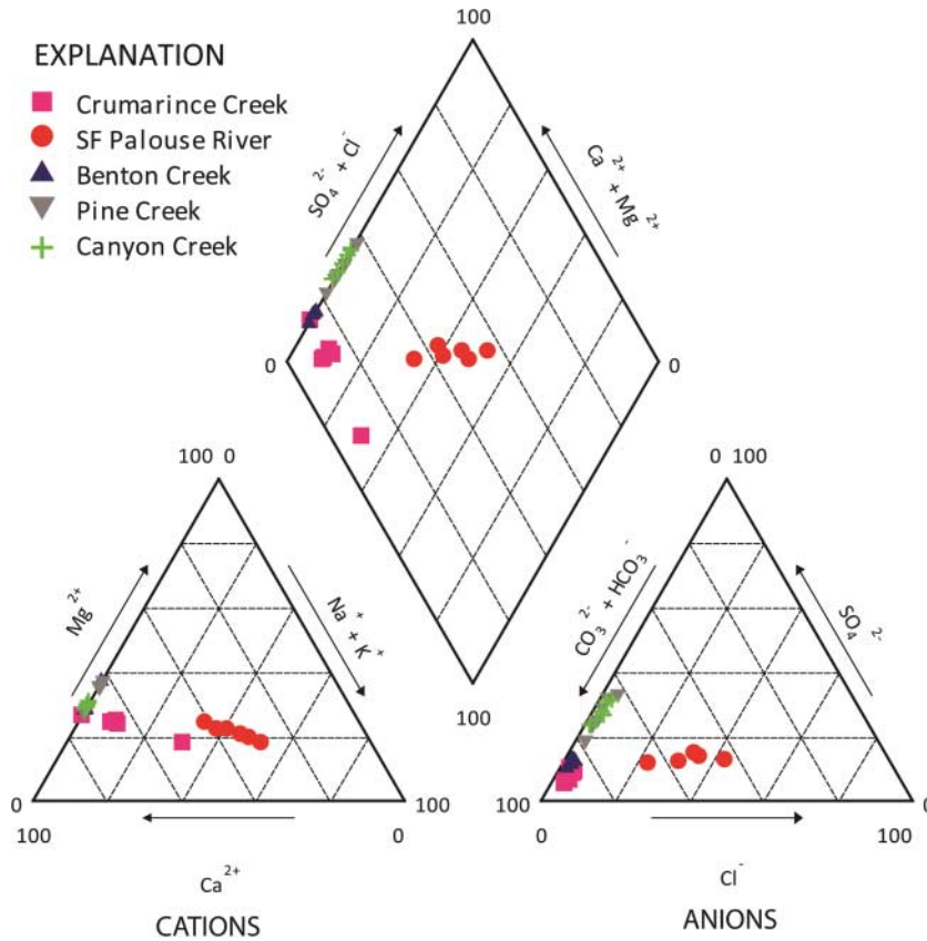
Figure 8. Piper diagram showing major ion composition in five watersheds in the inland PNW throughout the baseflow summer period in 2013.
