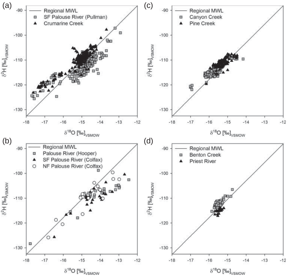
Figure 5. Isotopic composition of surface waters in the inland PNW, USA. The regional meteoric water line is plotted as reference ( \delta^2\text{H} = 7.42 \cdot \delta^{18}\text{O} + 0.88 ). (a) SF Palouse River (Pullman, WA): \delta^2\text{H} = 4.52 \cdot \delta^{18}\text{O} - 44.5 ; n = 195 , r^2 = 0.73 . Crumrine Creek (Moscow, ID): \delta^2\text{H} = 5.34 \cdot \delta^{18}\text{O} - 29.3 ; n = 245 , r^2 = 0.85 . (b) Palouse River (Hooper, WA): \delta^2\text{H} = 4.47 \cdot \delta^{18}\text{O} - 45.2 ; n = 24 , r^2 = 0.76 . SF Palouse River (Colfax, WA): \delta^2\text{H} = 5.02 \cdot \delta^{18}\text{O} - 38.1 ; n = 23 , r^2 = 0.88 . NF Palouse River (Colfax, WA): \delta^2\text{H} = 4.88 \cdot \delta^{18}\text{O} - 38.2 ; n = 23 , r^2 = 0.86 . (c) Canyon Creek (Wallace, ID): \delta^2\text{H} = 4.15 \cdot \delta^{18}\text{O} - 49.4 ; n = 158 , r^2 = 0.71 . Pine Creek (Pinehurst, ID): \delta^2\text{H} = 3.99 \cdot \delta^{18}\text{O} - 50.1 ; n = 143 , r^2 = 0.48 . (d) Benton Creek (Priest River, ID): \delta^2\text{H} = 6.09 \cdot \delta^{18}\text{O} - 18.02 ; n = 84 , r^2 = 0.66 . Priest River (Priest River, ID): \delta^2\text{H} = 4.57 \cdot \delta^{18}\text{O} - 44.5 ; n = 18 , r^2 = 0.38 .
