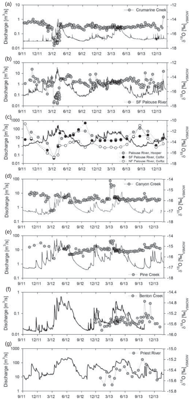
Figure 6. Time series of \delta^{18}\text{O} (‰) for surface water compared to discharge ( \text{m}^3/\text{s} ) at each outflow location (a) Crumarine Creek, Moscow Mountain, Idaho [ A = 6.35 \text{ km}^2 ]. (b) South Fork of the Palouse River, Pullman, Washington [ A = 342 \text{ km}^2 ]. (c) Palouse River (grey circles) [ A = 6,472 \text{ km}^2 ], Hooper, Washington; South Fork of the Palouse River (black circles) [ A = 709 \text{ km}^2 ], Colfax, Washington; North Fork of the Palouse River (open circles) [ A = 1287 \text{ km}^2 ], Colfax, Washington. Black line denotes the discharge of the Palouse River at Hooper, Washington. (d) Canyon Creek [ A = 60 \text{ km}^2 ], Wallace, Idaho. (e) Pine creek [ A = 190 \text{ km}^2 ], Pinehurst, Idaho. (f) Benton Creek [ A = 7.24 \text{ km}^2 ], Priest River, Idaho. (g) Lower Priest River [ A = 2,335 \text{ km}^2 ], Priest River, Idaho.
