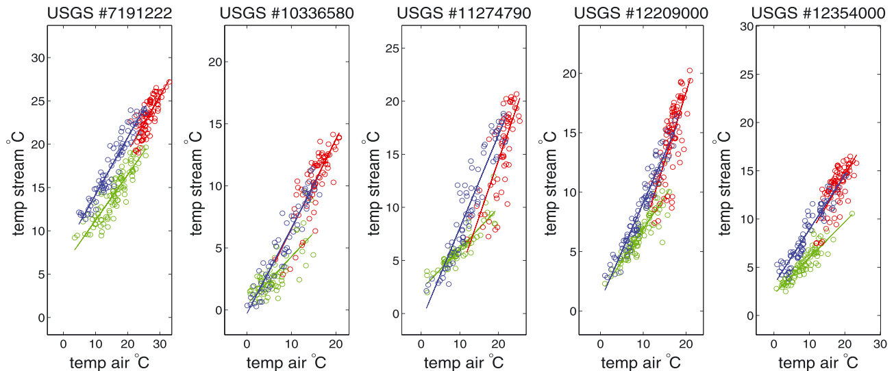
Figure 12. Examples of the linear model (LM) fitted to seasonal 7-day mean values of air ( t_a ) and stream ( t_s ) at five U.S. Geological Survey (USGS) sites: #07191222 (Beaty Creek near Jay, OK), #10336580 (Upper Truckee Rv at S Upper Truckee Rd near Meyers, CA), #11274790 (Tuolumne R A Grand Canyon of Tuolumne Ab Hetch Hetchy, CA), #12209000 (SF Nooksack River near Wickersham, WA) and # 12354000 (St Regis River near St Regis, MT). Green, red and blue markers are spring, summer and fall, respectively
