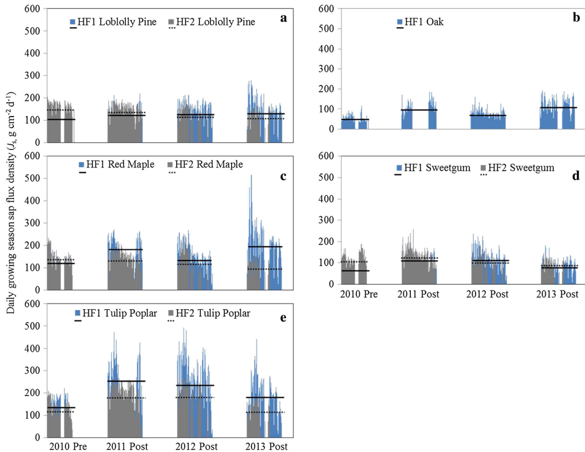
Figure 5. Daily growing season sap flux density between treatment (HF1) and reference (HF2) watersheds during preharvest (201) and postharvest (2011–2013) periods across (a) loblolly pine, (b) oak, (c) red maple, (d) sweetgum, and (e) tulip poplar. Solid line is growing season (May–October) mean J_s in HF1, and dash line is growing season mean J_s in HF2. Gaps in data are because of sap flow sensor errors or battery recharge issues. Pre = preharvest; Post = postharvest
