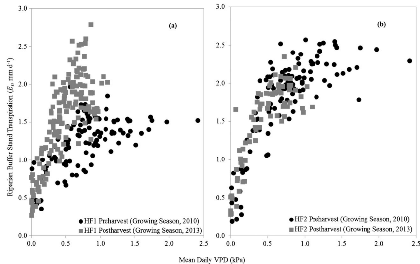
Figure 8. Relationships between mean daily vapour pressure deficit (VPD) and riparian buffer stand transpiration ( E_s ) in (a) treatment (HF1) and (b) reference (HF2) watersheds during growing season (May–October) in preharvest (2010) and postharvest (2013) periods
