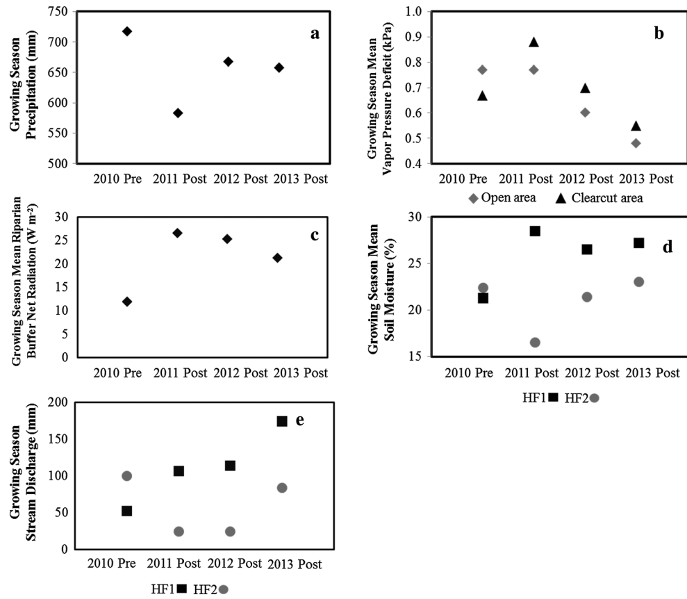
Figure 4. Growing season (May–October) (a) precipitation, (b) open area and clearcut area vapour pressure deficit (VPD), (c) riparian buffer net radiation, (d) soil moisture, and (e) stream discharge in treatment (HF1) and reference (HF2) watersheds over preharvest (2010) and postharvest (2011–2013) periods. Soil moisture sensors were installed in June 2010; thus, 2010 preharvest soil moisture growing season data covers June–October. Pre = preharvest; Post = postharvest
