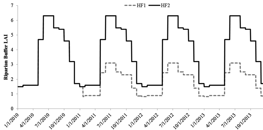
Figure 3. Preharvest (2010) and postharvest (2011–2013) riparian buffer leaf area index (LAI) in treatment (HF1) and reference (HF2) watersheds. Riparian buffer LAI was only measured in 2013. As indicated in Figure 2, riparian buffer percent canopy cover did not change significantly in reference watersheds (HF2) from 2009 to 2013 and in treatment watersheds (HF1) from 2011 to 2013. Therefore, we applied 2013 LAI values to previous years to depict canopy openness
